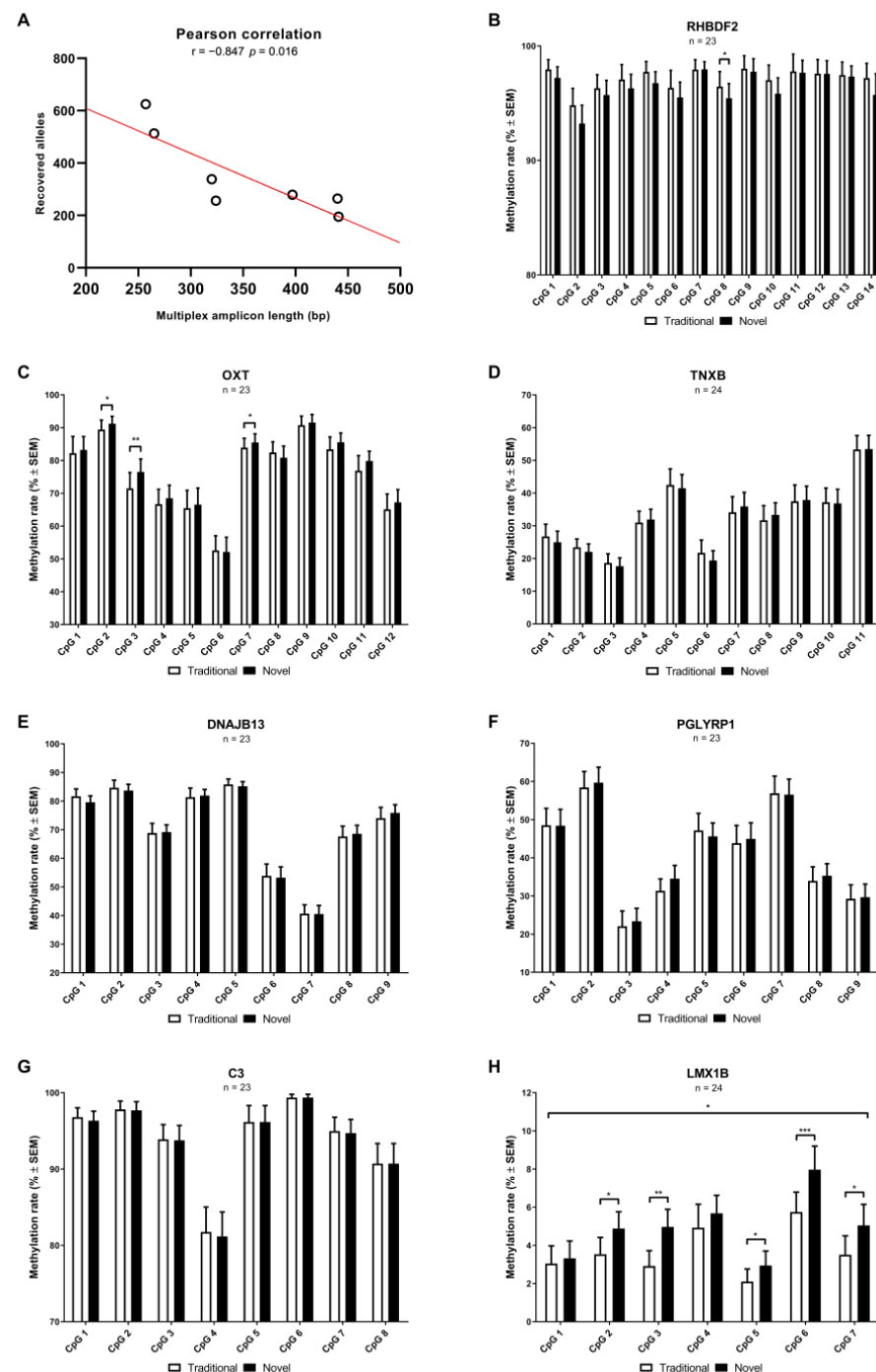
Figure 2. (A) Displayed is the Pearson correlation test was performed to assess whether there was a correlation between the number of recovered alleles and multiplex amplicon length of each gene. (B–H) Shown for each target gene are the paired cytosine-phosphate-guanine (CpG) methylation rates (mean percentage \pm standard error of the mean [SEM]) estimated by both the traditional and novel downstream data analysis for limiting dilution bisulfite pyrosequencing (LDBSP) on pools of 50 neurons. A one-way repeated measures multivariate analysis of variance (MANOVA) was performed in order to determine whether there was a combined significant difference in the CpG methylation rates estimated by both methods. Subsequently, a univariate analysis was performed in order to identify differences between the methylation rates for each individual CpG site. A p -value of <0.05 was considered statistically significant. Significant findings for the multivariate and univariate tests are indicated with an asterisk (* = p < 0.05 ; ** = p < 0.01 ; *** = p < 0.001 ).
