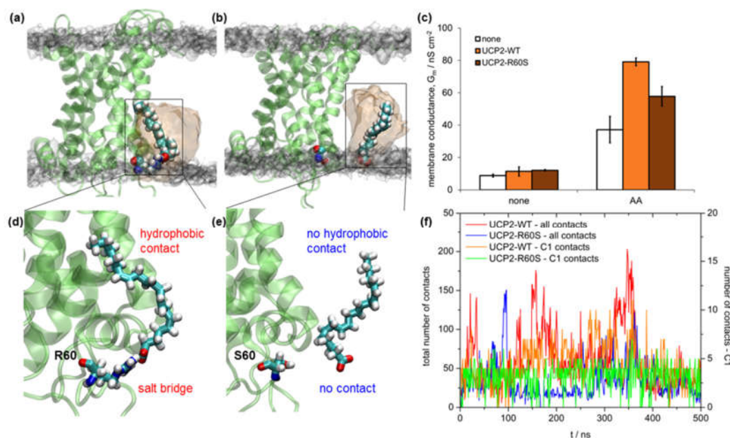
Figure 8. Snapshots of 500 ns simulations of UCP2 homology modeled structures (UCP2h) with added arachidonic acid anion ( \text{AA}^- ). A starting structure of protein used for binding calculations is taken from UCP2h MD simulations after 2 \mu\text{s} . UCP2h structure with \text{AA}^- (a) bound to R60 and (b) not bound to the mutated binding site S60. A volume map of phosphorus atoms of DOPC lipid is presented in transparent gray color (surface isovalue set to 0.0064) and volume map of \text{AA}^- is presented in transparent orange color (surface isovalue set to 0.02). (c) Specific membrane conductance of lipid bilayers in the absence of protein (white), and presence of UCP2-WT (orange) or UCP2-R60S (brown). Membranes were made of 45:45:10 mol.% DOPC:DOPE:CL reconstituted with 15 mol.% \text{AA}^- where indicated. Lipid and protein concentrations were 1.5 mg/mL and 4 \mu\text{g} per mg of lipid, respectively. The buffer solution contained 50 mM \text{Na}_2\text{SO}_4 , 10 mM TRIS, 10 mM MES and 0.6 mM EGTA at pH = 7.34 and T = 306 K. Data are represented as the mean and standard deviation from three independent experiments. (d) Zoomed region of \text{AA}^- binding to UCP2h structure. (e) Zoomed region of \text{AA}^- binding to UCP2-R60S mutant structure. (f) Total number of contacts within 0.35 nm between all \text{AA}^- atoms and UCP2-WT and (red color) and UCP2-R60S mutant structures (blue color), respectively. Total number of contacts within 0.35 nm between \text{AA}^- carboxyl atom towards UCP2h (orange color) and UCP2-R60S structures (green color).
