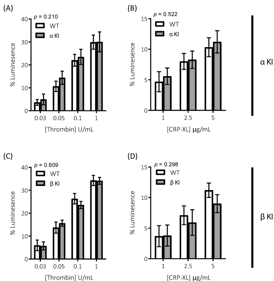
Figure 5. Secretion of the \delta -granule cargo ATP is unaltered in platelets expressing phosphorylation-resistant GSK3 \alpha or GSK3 \beta . ATP secretion from platelets was monitored using CHRONOLUME ® and the Infinite ® 200 PRO multimode reader (TECAN, Reading, UK). Platelets from \alpha KI mice had no significant alterations in ATP secretion in response to (A) thrombin or (B) CRP-XL ( n = 5 ). Platelets from \beta KI mice had no significant alterations in ATP secretion in response to (C) thrombin or (D) CRP-XL ( n = 5 ). A 2-way ANOVA (Variable 1 = genotype, Variable 2 = concentration of agonist) was used to test for differences between groups. Data are the peak luminescence expressed as a % of luminescence signal evoked by a fixed concentration of ATP.
