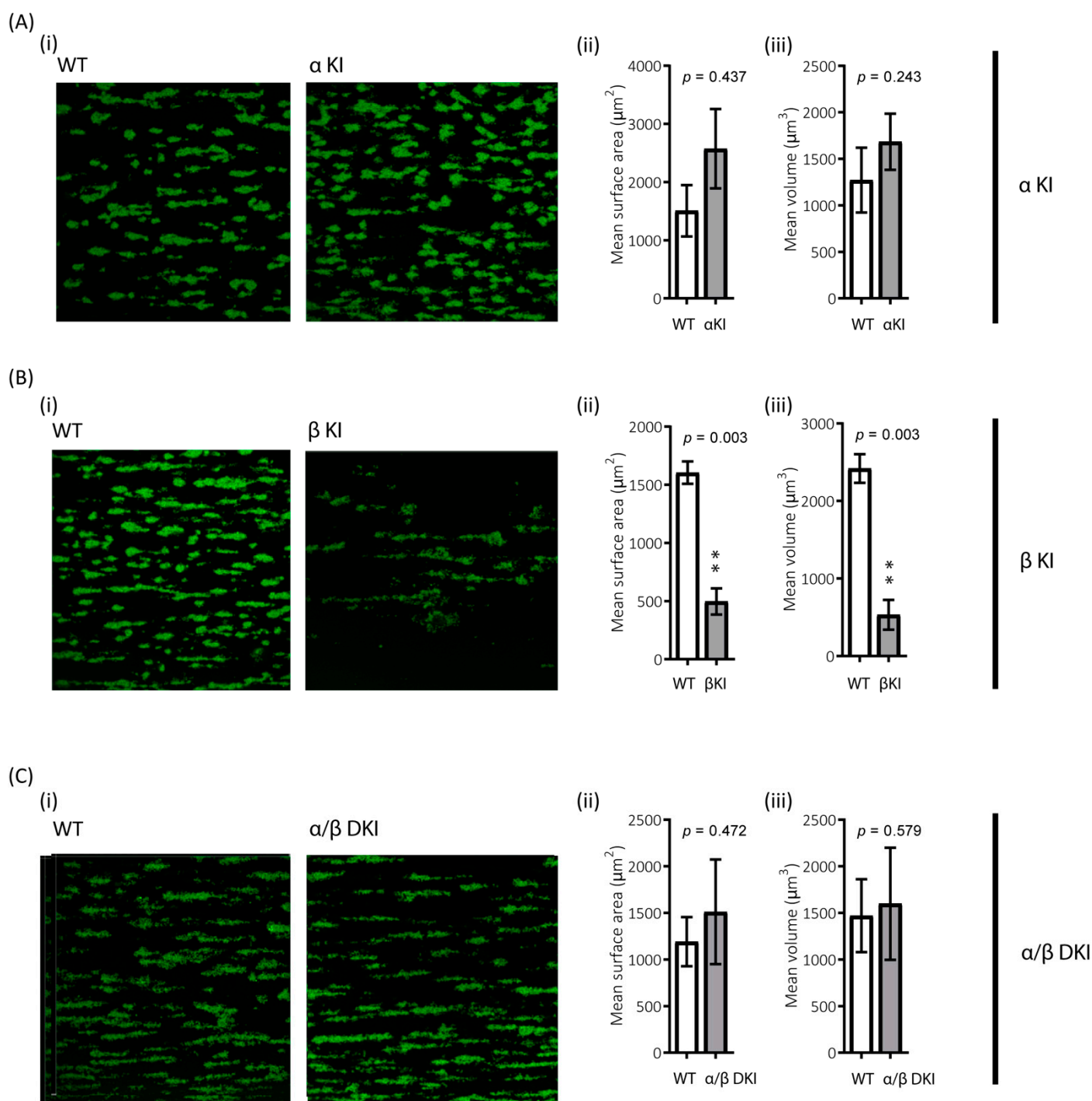
Figure 8. Reduced platelet accumulation on collagen under shear in blood from phosphorylation-resistant GSK3 \beta mice. Whole anticoagulated blood was flowed at 1000 s ^{-1} over fibrillar collagen coated Ibidi ^{\circ} \mu -slides (for parallel flow assays): (A) Blood from \alpha KI mice exhibited similar amount of platelet deposition compared to WT controls ( n = 12 ). In contrast (B) Blood from \beta KI mice exhibited reduced platelet deposition compared to WT controls ( n = 7 ). (C) Blood from \alpha/\beta DKI mice exhibited similar amount of platelet deposition compared to WT controls ( n = 10 ). Thrombus formation was quantified from fixed samples (end-point) by imaging 5 randomly chosen fields of view using a Leica SP5-II confocal laser scanning microscope attached to a Leica DMI 6000 inverted epifluorescence microscope (Leica Microsystems, United Kingdom). Data are representative images, and quantification of surface area covered \mu\text{m}^2 and total thrombus volume \mu\text{m}^3 . Student's t-test was used to test for statistical differences between genotypes **: p < 0.01 .
