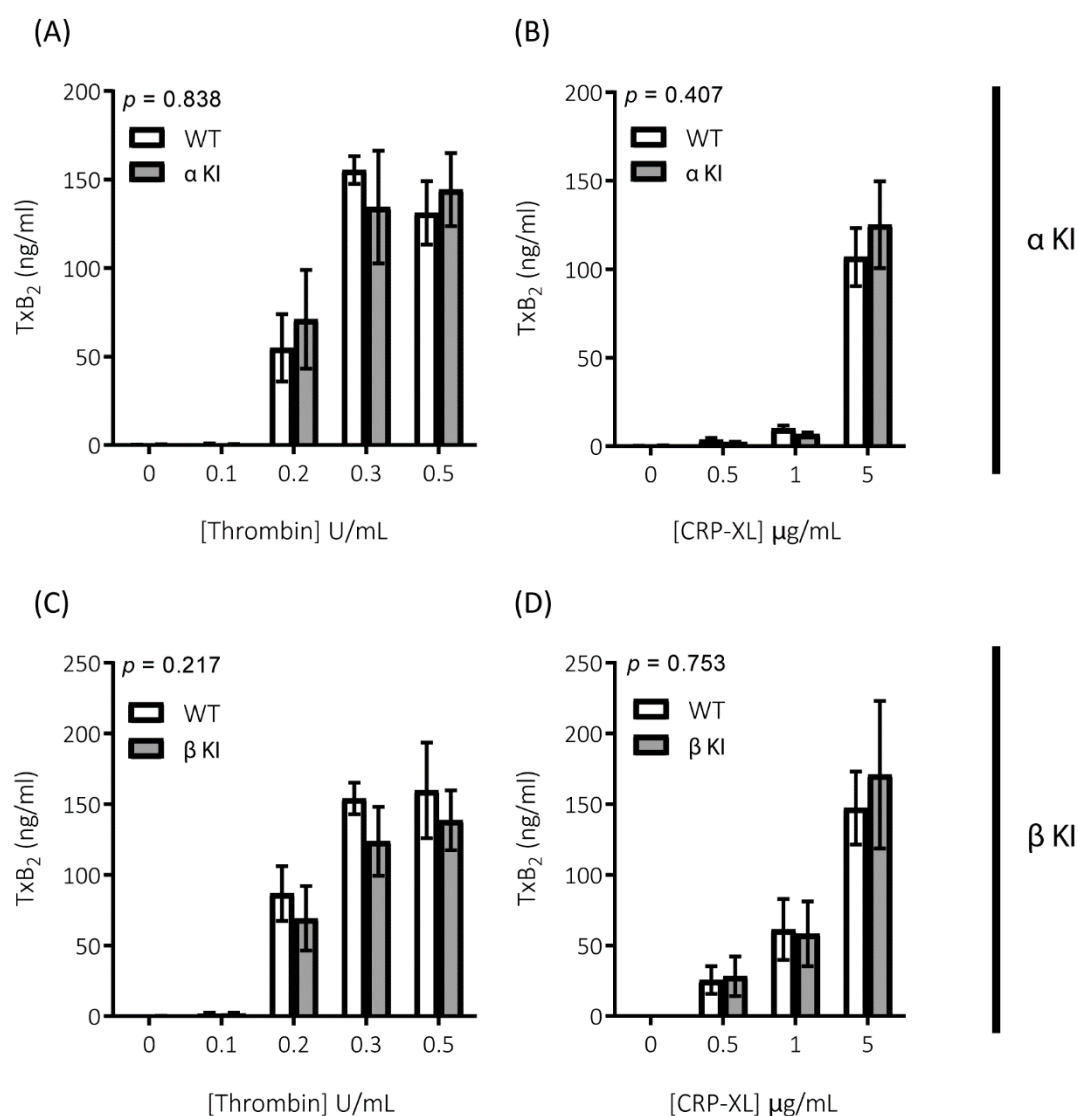
Figure 6. Generation of \text{TxA}_2 is unaltered in platelets expressing phosphorylation-resistant GSK3 \alpha or GSK3 \beta . \text{TxA}_2 generation was determined by measuring the concentration of \text{TxB}_2 in platelet supernatants using a \text{TxB}_2 ELISA kit. Platelets from \alpha KI mice had no significant alterations in \text{TxA}_2 generation in response to (A) thrombin or (B) CRP-XL ( n = 4 ). Platelets from \beta KI mice had no significant alterations in \text{TxA}_2 generation in response to (C) thrombin or (D) CRP-XL ( n = 4 ). A 2-way ANOVA (Variable 1 = genotype, Variable 2 = concentration of agonist) was used to test for differences between groups. p -values are indicated in figure. Data are expressed as ng/mL \text{TxB}_2 determined from standard curve.
