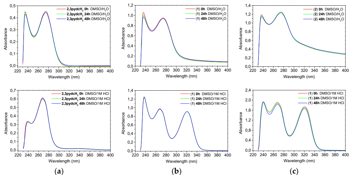
Figure 10. Time-dependent (0 h, 24 h and 48 h) stability studies on: (a) 2,3pydcH 2 , (b) complex 1, (c) complex 2 in DMSO/H 2 O 1:50 (v/v) (top) and DMSO/1M HCl 1:50 (v/v) (bottom) solutions monitored by UV-Vis absorption spectra.
