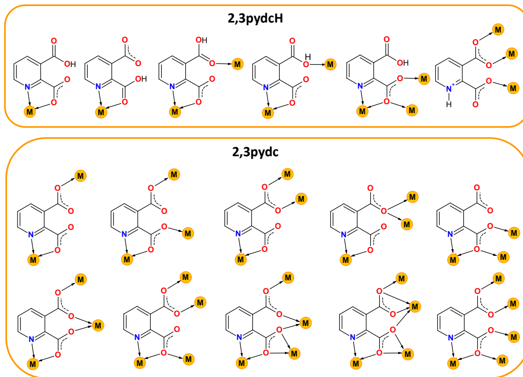
Scheme 1. Selected coordination modes of mono-deprotonated-2,3pydcH (top) and deprotonated-2,3pydc (bottom) forms of pyridine-2,3-dicarboxylic acid (2,3pydcH 2 ) in coordination with different metal ions reported in the literature [43–55].
