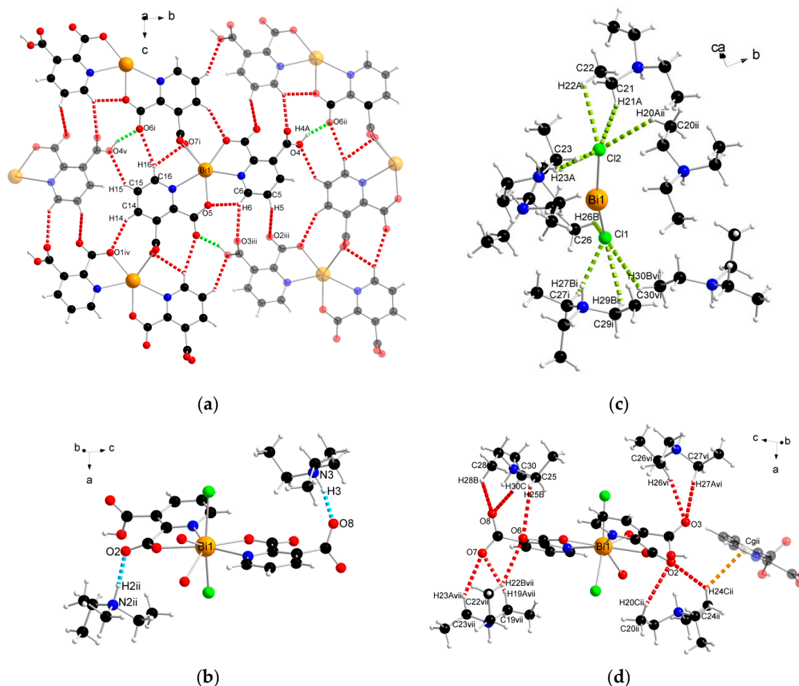
Figure 6. The geometry of noncovalent interactions in complex 2: (a) O/C-H...O formed between adjacent polymeric chains, (b) N-H...O, (c) C-H...Cl and (d) C-H...O/π formed between Et 3 NH cations and polymeric chains (translucent molecules belong to adjacent chains) (Bi—orange, O—red, N—blue, Cl—green, C—black, H—white).
