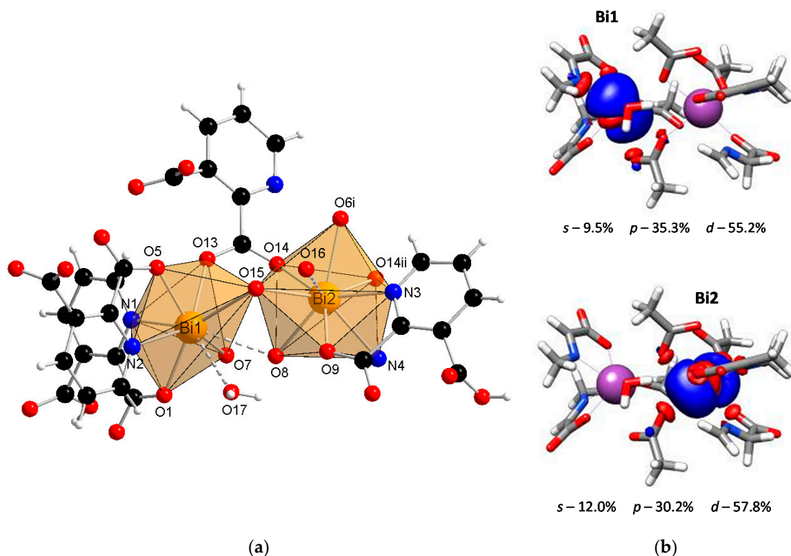
Figure 1. (a) The molecular structure with an atom numbering scheme of complex 1 (Symmetry codes: (i) -x, 1-y, 1-z ; (ii) 1-x, 1-y, 1-z ) (Bi—orange, O—red, N—blue, C—black, H—white); (b)
