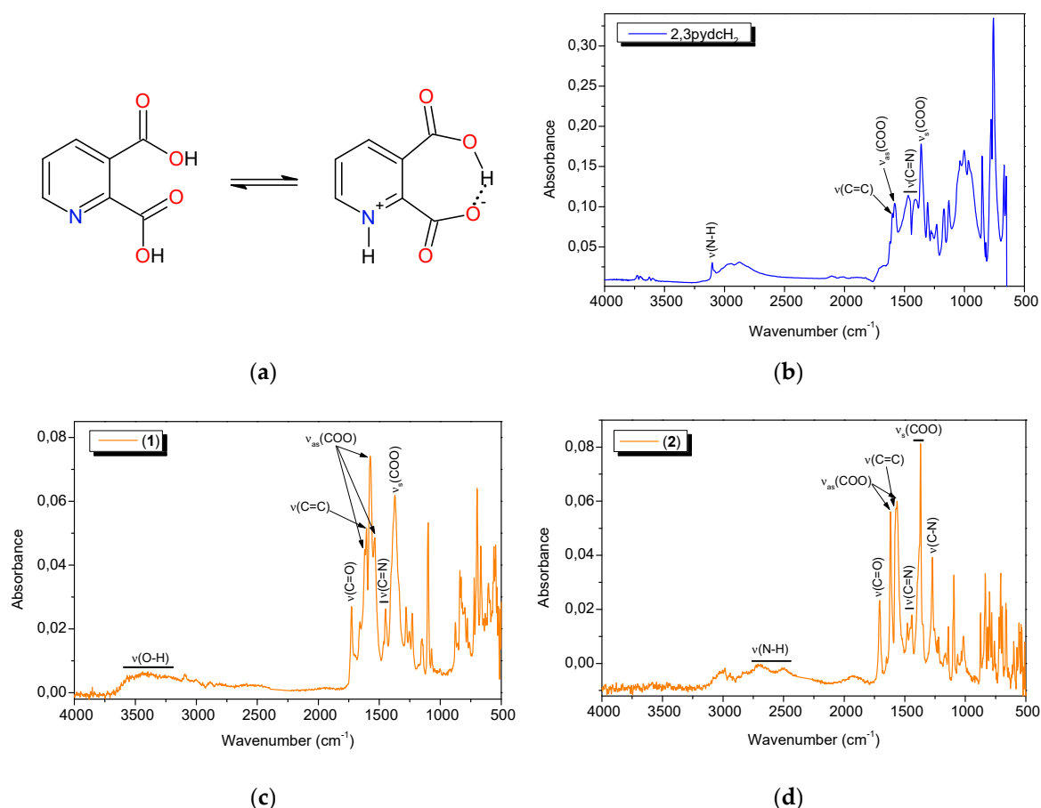
Figure 7. (a) The non-zwitterionic and zwitterionic form of 2,3pydcH 2 ; the FT-IR spectra of: (b) 2,3pydcH 2 , (c) complex 1 and (d) complex 2.
