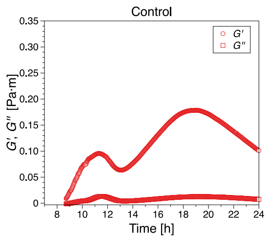
Figure S1. Dynamic moduli, G' and G'' , of the Control biofilm grown for the strain sweep test in Figure 8. Note the pronounced decrease in dynamic moduli in region IV, decrease that was not accounted for in the standard deviation calculations in Figure 2.
