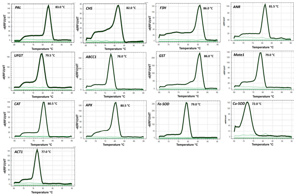
Figure 1. The bold lines are the melt curves for the amplicons and the thin lines are the melt curves for the primers (all are basal). Each primer represented the amplicon size, melting temperature and qPCR efficiency > 90%.
