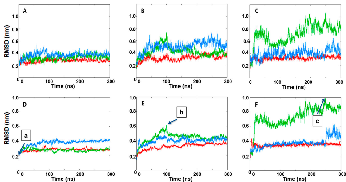
Figure 5. The RMSDs of IRE1 face-to-face dimer C \alpha atoms during the three MD simulation replicas of (A) a native face-to-face crystal dimer structure (PDB code: 3P23), (B) KIRA docked in PDB 3P23 dimer, (C) protein–protein docked pose of PDB 4U6R in the face-to-face dimer form. Interface RMSDs of IRE1 face-to-face dimer C \alpha atoms during the three MD simulation replicas of (D) a native face-to-face crystal dimer structure (PDB code: 3P23), (E) KIRA docked in PDB 3P23 dimer, (F) protein–protein docked pose of PDB 4U6R in the face-to-face dimer form. Replicas 1, 2, and 3 are represented in red, green, and blue, respectively. Individual frames of the MD simulations labeled (a), (b), and (c) are shown in Figure S4.
