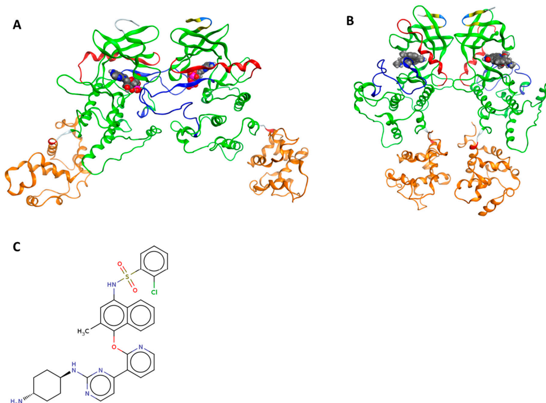
Figure 1. Ribbon diagram representing the dimeric structures of the inositol-requiring enzyme 1α (IRE1) cytosolic regions. (A) Face-to-face dimer (PDB 3P23). (B) Back-to-back arrangement (PDB 4YZC). The kinase domain is shown in green (residues 571–832), the helix-αC in red (residues 603–623), the activation segment in blue (residues: 711–741), the RNase domain in orange (residues 837–963). The yellow segment represents the β-strand and the cyan the H-bonded turn that are not part of the kinase or RNase domain. ADP and staurosporine are highlighted in spaces filling models in (A) and (B), respectively, to indicate the kinase binding sites. (C) 2D molecular representation of Kinase inhibiting RNase attenuators (KIRA).
