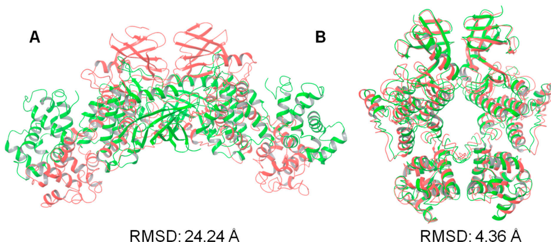
Figure 4. Illustration of the protein–protein docking results of KIRA-containing IRE1 monomers (PDB code: 4U6R). Values shown are the RMSD in angstrom of the positions of the C \alpha atoms of the best-scoring docked pose (green) against the native IRE1 dimer structure in (A) face-to-face (PDB code: 3P23) and (B) back-to-back (PDB code: 4YZC) conformation (red).
