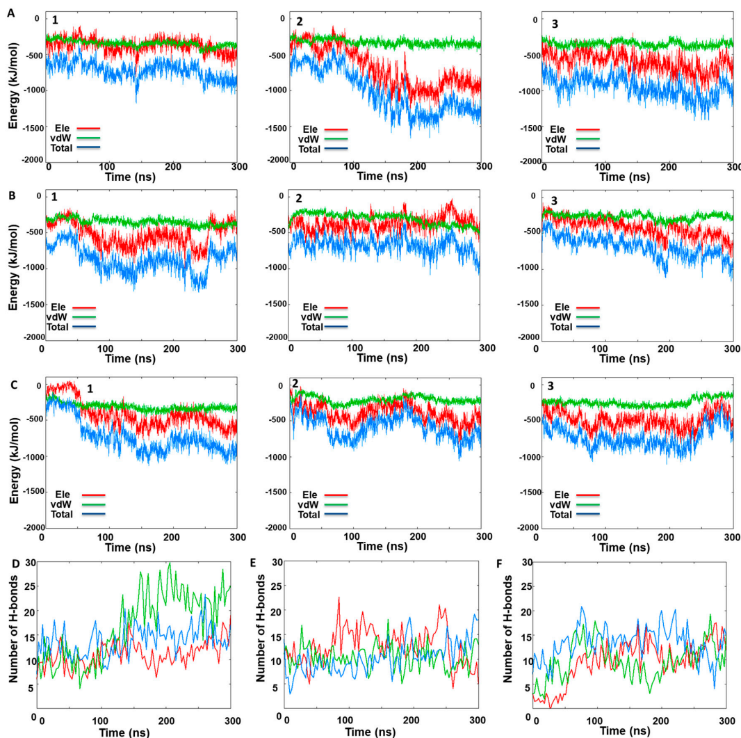
Figure 6. IRE1 face-to-face dimer MD simulations. Time-dependent interaction energy profiles for monomer A with monomer B during the three MD simulation replicas of (A) native face-to-face crystal dimer (PDB code: 3P23), (B) KIRA-docked face-to-face dimer (PDB code: 3P23), (C) protein–protein docked pose of PDB 4U6R in the face-to-face dimer form. Hydrogen bond analysis between monomers A and B during three MD replicas for (D) native face-to-face crystal dimer (PDB code: 3P23), (E) KIRA-docked face-to-face dimer (PDB code: 3P23), (F) protein–protein docked pose of PDB 4U6R in the face-to-face dimer form.
