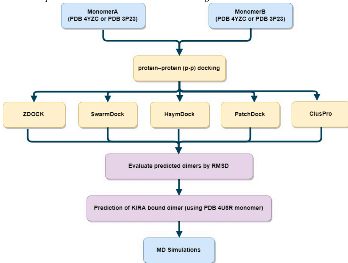
Figure 2. Schematic representation of the protein-protein docking scheme used for predicting KIRA-bound dimer structures. RMSD stands for the root mean square deviation calculated for C \alpha atoms by superposing the docked structure with the crystallographic structure.
