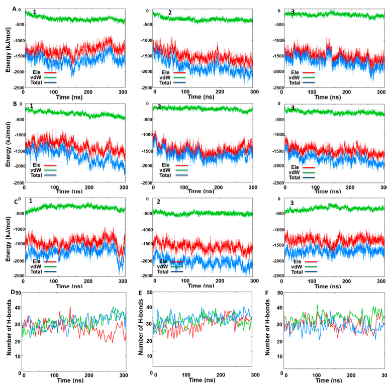
Figure 8. IRE1 back-to-back dimer MD simulation data for the three MD replicas. Time-dependent interaction energy profiles for monomer A with monomer B during the MD simulations of (A) native back-to-back dimer (PDB code: 4YZC), (B) KIRA docked in the 4YZC structure, and (C) protein–protein docked pose of PDB 4U6R in the back-to-back dimer. Hydrogen bond analysis between the
