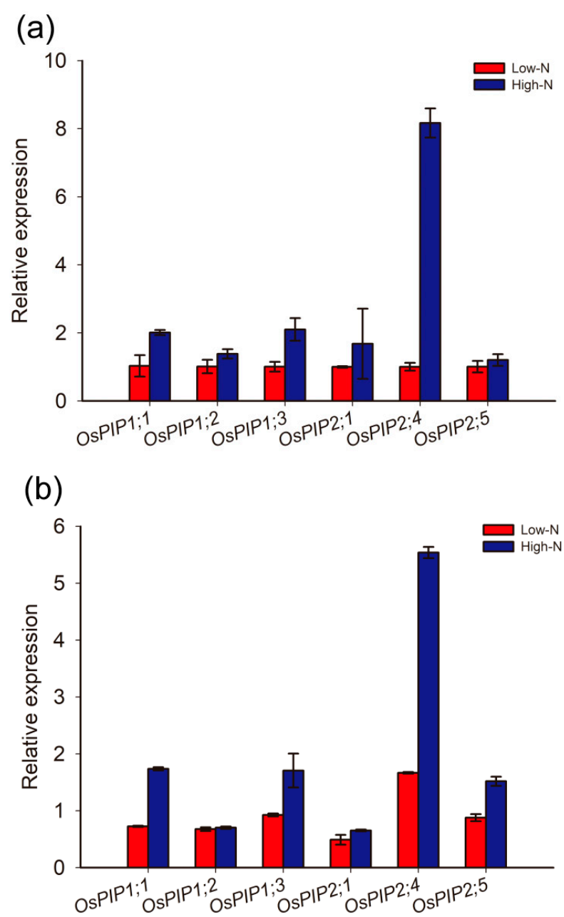
Figure S2. The expression of PIPs in roots supply with Low-N and High-N in SY63 and YD6.
