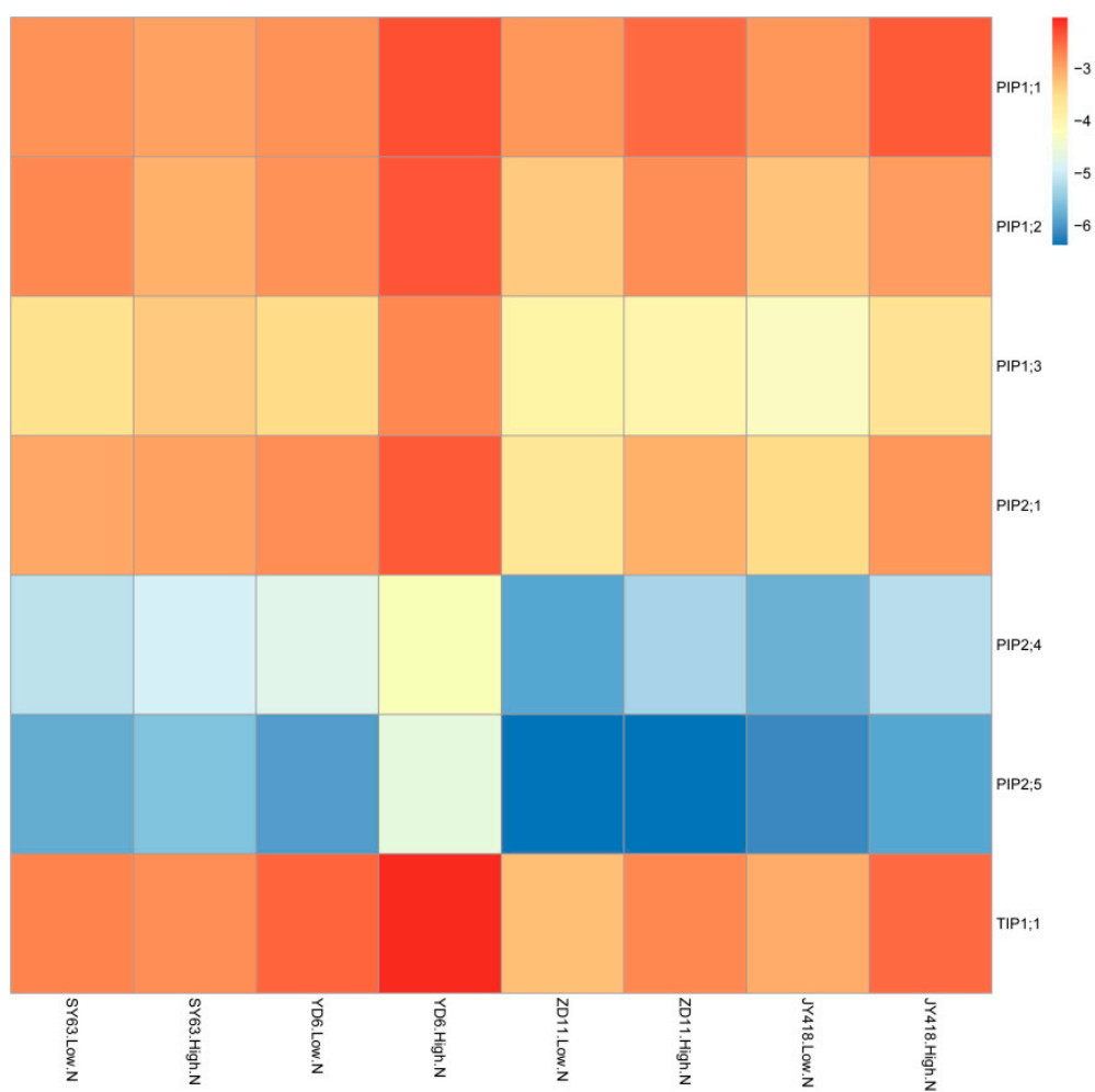
Figure S1. The expressions of six PIPs and one TIP in leaves supply with Low-N and High-N in four rice cultivars.
