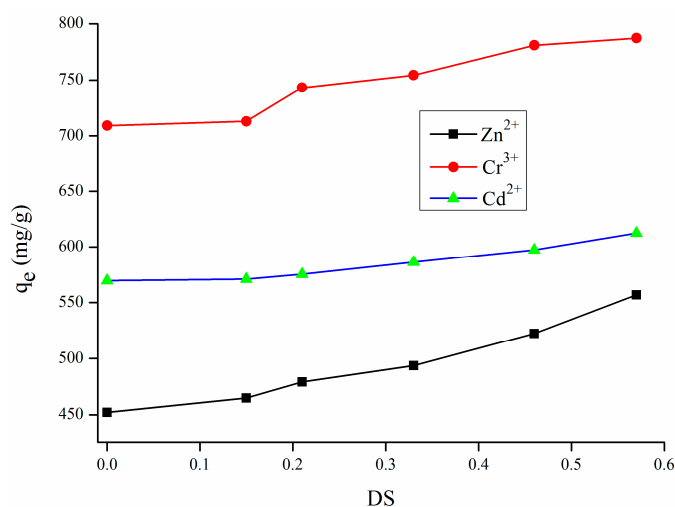
Figure 6. Effect of DS on the hydrogel adsorption for xylan-chain-g-acrylic acid (CAX-g-AA) hydrogel.
