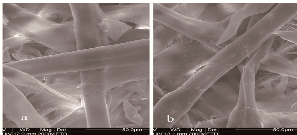
Figure 4. SEM of hand sheets of alkaline peroxide mechanical pulp (APMP) pulp/chemical pulp (1:1) without additives (a) and with the addition of CAX (b).
