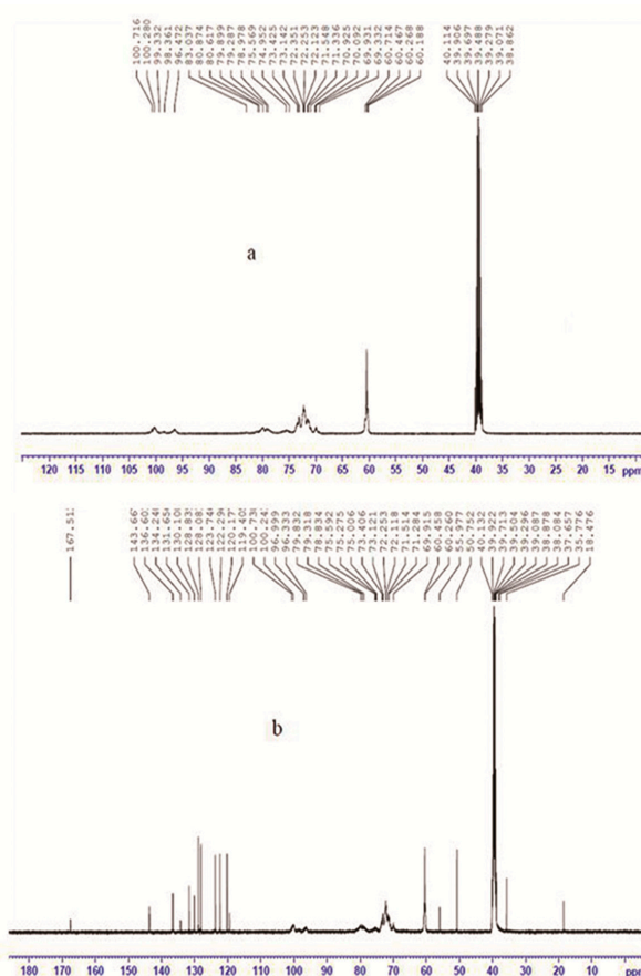
Figure 2. ^{13}\text{C} -NMR spectra of xylan (spectrum (a)) and CAX (spectrum (b), sample 17 in Table 1).
