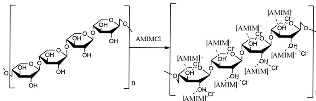
Scheme 1. Proposed dissolution mechanism of xylan in 1-allyl-3-methylimidazolium chloride (AMIMCl).
