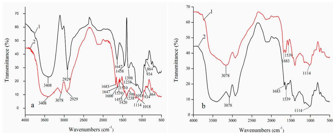
Figure 1. (a) FT-IR spectra of xylan (spectrum 1) and CAX (spectrum 2, sample 17 in Table 1); (b) FT-IR spectra of CAX with different DSs (spectrum 1, sample 17; and spectrum 2, sample 18).
