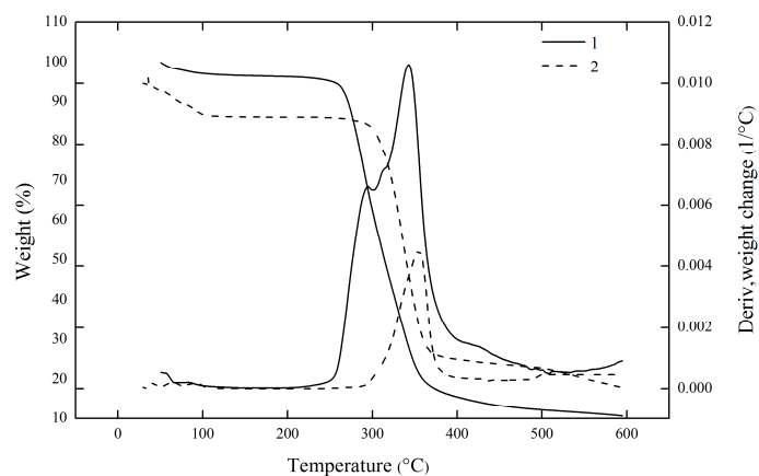
Figure 3. TGA/DTA curves of CAX (curve 1, sample 17 in Table 1) and xylan (curve 2).
