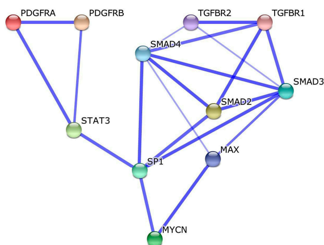
Figure 8. Identification of molecular pathways linking PDGFC (platelet derived growth factor C) and TGFB1 (transforming growth factor \beta 1) to MYCN (MYCN proto-oncogene, bHLH transcription factor). A meta-analysis of the human interactome was performed to determine whether signaling pathways could link MYCN (a known repressor of NDRG1 expression) to the identified candidate
