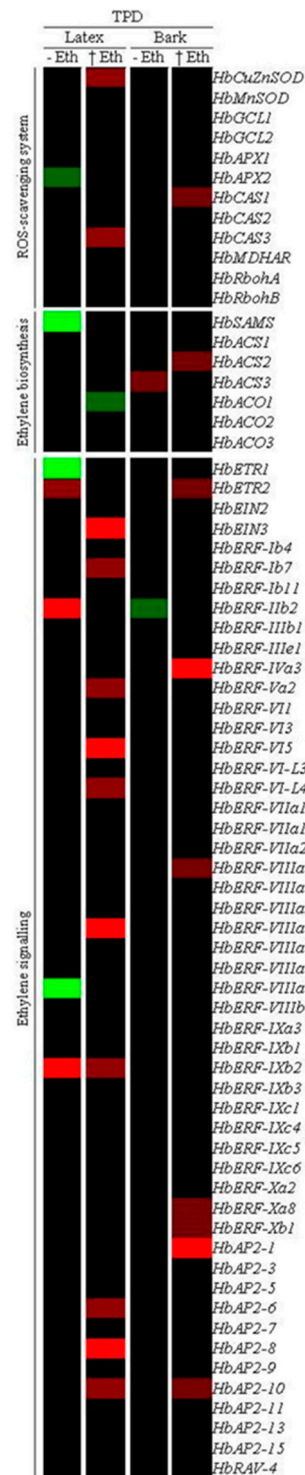
Figure 9. Fold change profile of 70 genes of Hevea brasiliensis involved in reactive oxygen species (ROS)-scavenging system, ethylene biosynthesis and signalling during the occurrence of Tapping Panel Dryness (TPD) in 6-year-old mature trees. Values are ratio between TPD and healthy plants without (–Eth) or with ethephon (+Eth) stimulation for six biological replicates. Values of relatives transcript abundance was performed with an ANOVA followed by the Student Newman–Keuls test. Upregulated genes were shown in bright red for a threshold value \geq 5 ; dark red for value < 5 , and down-regulated genes were shown in bright green for a threshold value \leq 0.2 ; dark green for value > 0.2 . The non-significant genes are shown in dark colour.
