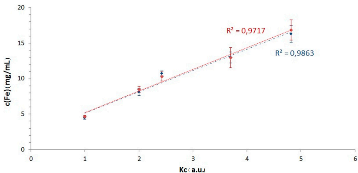
Figure S2. Comparison of iron content measurements with UV-VIS and MP-AES. SEON LA-BSA samples with different concentration factors K_C were measured by UV-VIS (Red dots and regression line) and MP-AES (Blue dots and regression line). All measurements were performed in triplicates. The values are displayed as mean \pm standard deviation.
