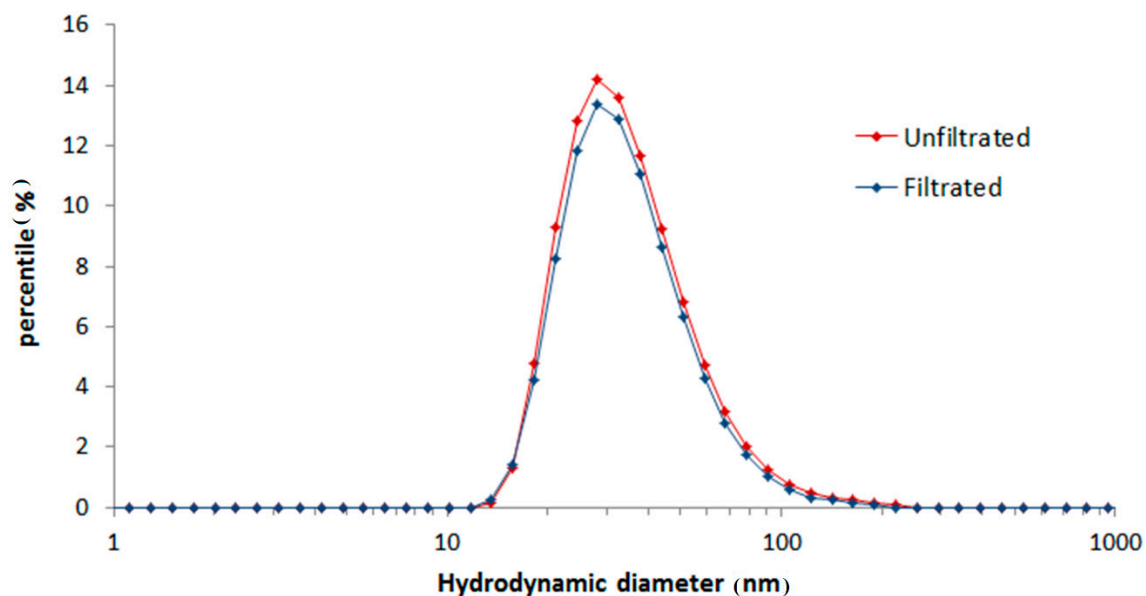
Figure S1. Size distribution of SEON LA-BSA at pH 7 before (red dots) and after (blue dots) filtration. Both samples are displayed as distribution by volume. The dots represent the mean of n = 3 individual measurements. The lines are drawn to guide the eye.
