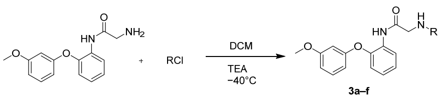
Scheme 4. Synthesis scheme for compounds 3a–f .
