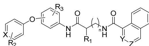
Figure 2. Core structure of known studied analogs of AOH1996.
