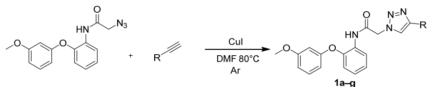
Scheme 2. Synthesis scheme for compounds 1a–g .
