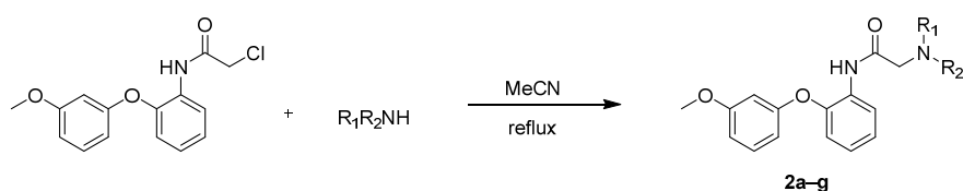
Scheme 3. Synthesis scheme for compounds 2a–g .
