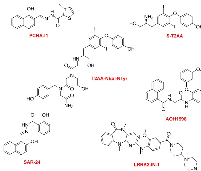
Figure 1. Examples of small-molecule PCNA inhibitors.
