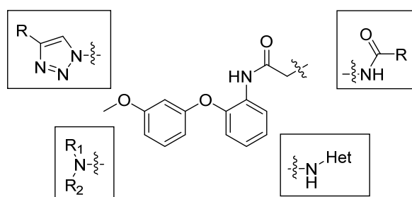
Scheme 1. Novel modifications to the core scaffold described herein.
