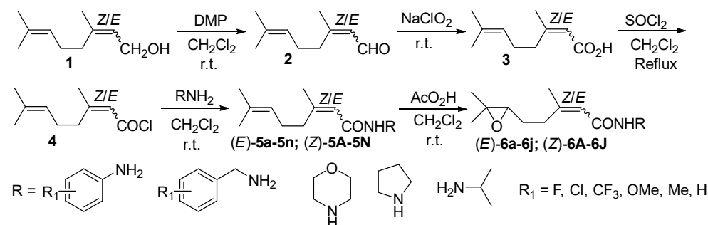
Scheme 2. Synthetic route of (Z/E)-3,7-dimethyl-2,6-octadienamide and their 6,7-epoxy analogues.
