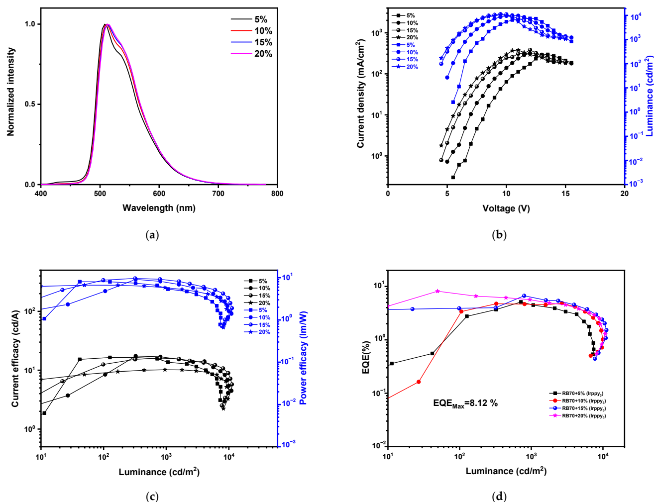
Figure 6. Characteristics of OLEDs using host material RB70 with different concentrations of emitter Ir(ppy) 3 . (a) Electroluminescence spectra, (b) current density–voltage–luminance, (c) current efficacy–luminance–power efficacy, (d) external quantum efficiency–luminance.
