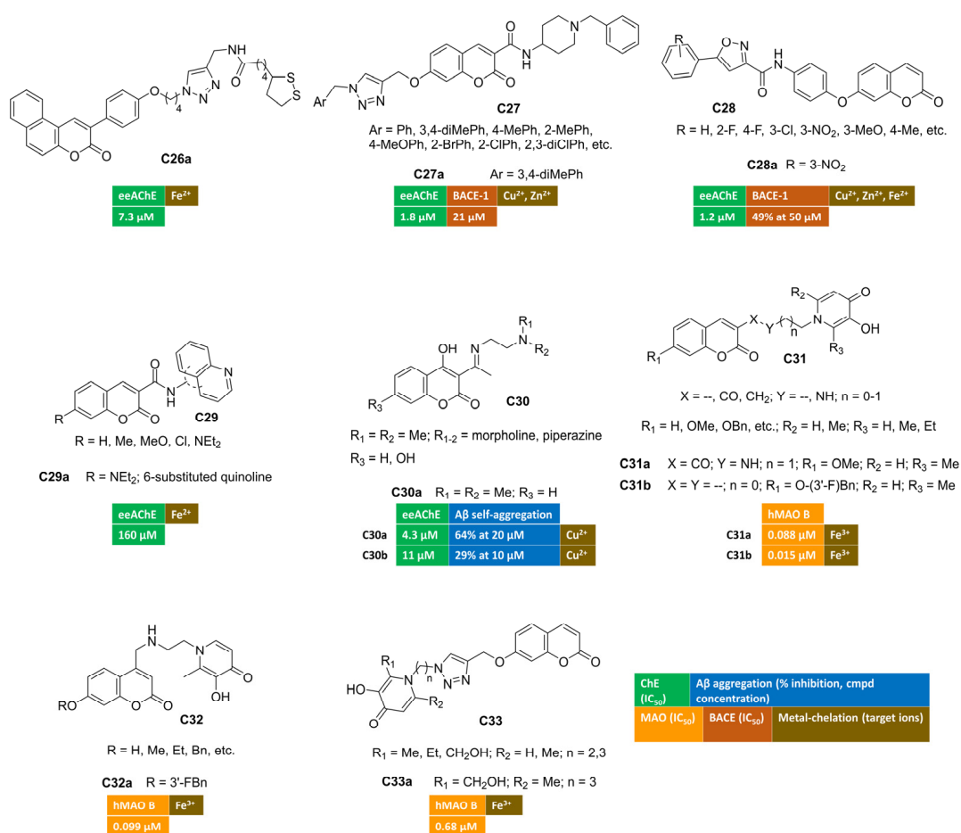
Figure 5. Metal-chelating multitarget coumarin derivatives C26–33 .
