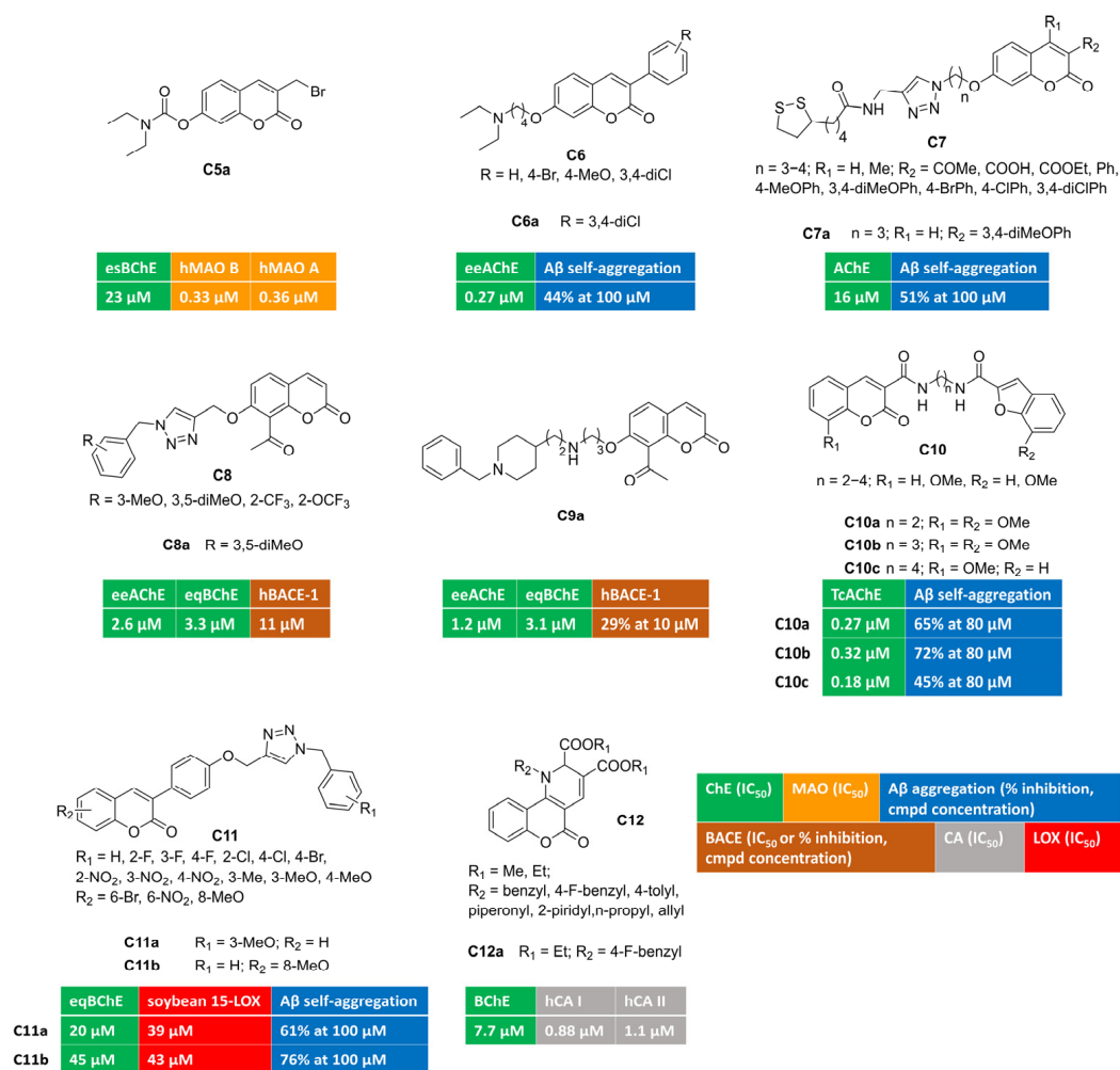
Figure 2. 3,7-, 7,8-, 3,6-, 3,8-, 3,4-Disubstituted and 3,4-fused multitarget coumarin derivatives C5–12 .
