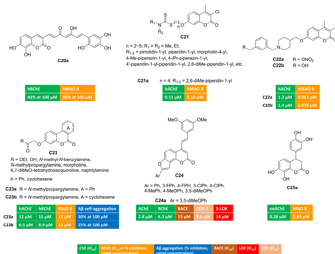
Figure 4. Polysubstituted multitarget coumarin derivatives C20–25 .
