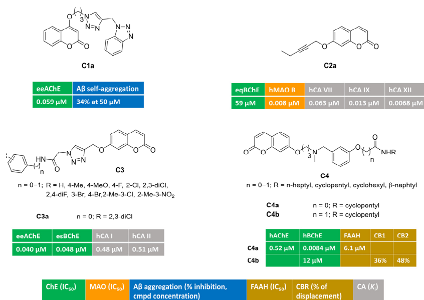
Figure 1. Monosubstituted multitarget coumarin derivatives C1–4 .
