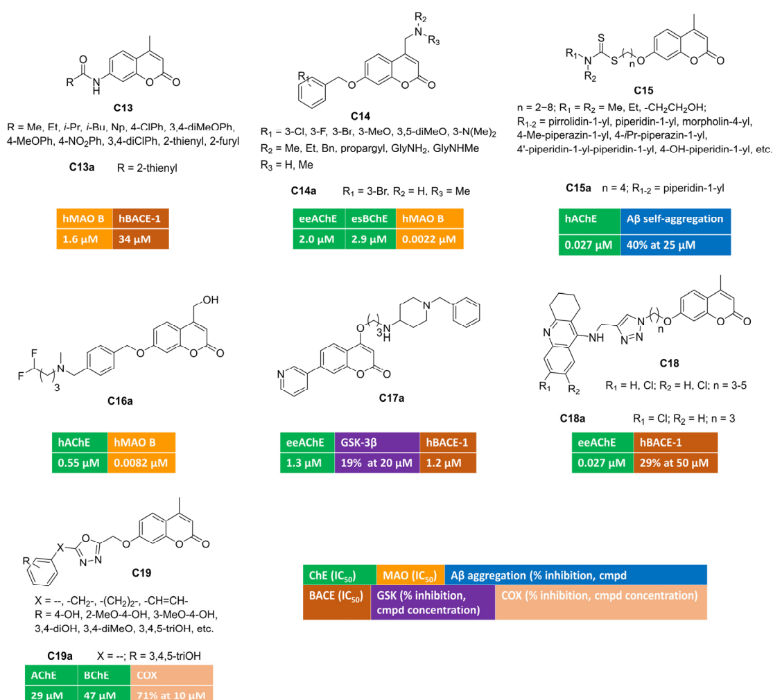
Figure 3. 4,7-Disubstituted multitarget coumarin derivatives C13–19 .
