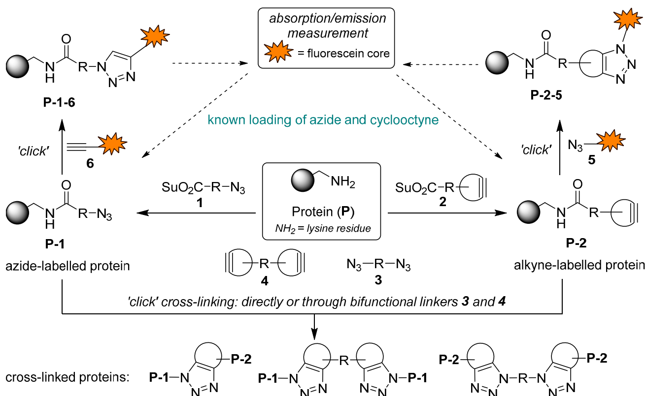
Figure 1. The planned method for studying covalent binding of native proteins.
