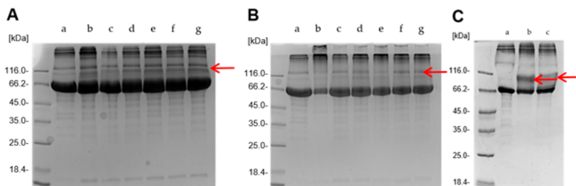
Figure 4. (A): SDS-PAGE of (a) BSA control, (b) BSA-2a + BSA-1b (1:1), (c) BSA-2a + BSA-1e (1:1), (d) BSA-2a + BSA-1a (1:1), (e) BSA-2a + BSA-1b (1:5), (f) BSA-2a + BSA-1e (1:5), and (g) BSA-2a + BSA-1a (1:5). (B): SDS-PAGE of (a) BSA control, (b) BSA-2c + BSA-1b (1:1), (c) BSA-2c + BSA-1e (1:1), (d) BSA-2c + BSA-1a (1:1), (e) BSA-2c + BSA-1b (1:5), (f) BSA-2c + BSA-1e (1:5), and (g) BSA-2c + BSA-1a (1:5). (C): SDS-PAGE of (a) BSA control, (b) BSA-2c + 3 (2:1), and (c) BSA-1b + 4 (2:1). (A–C): Detection after staining with Coomassie Brilliant Blue using the corresponding detection settings. Red arrows point to smeared spots at ~120 kDa corresponding to dimers of BSA.
