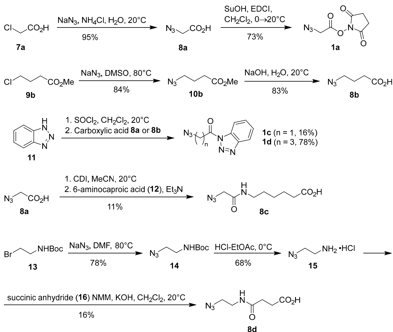
Scheme 1. Synthesis of azido acids 8a–d and azide-functionalized acylation reagents 1a,c,d .
