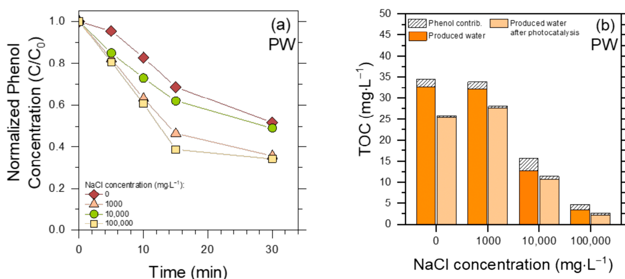
Figure 7. (a) Phenol degradation profiles in raw PW at different initial concentrations of NaCl, upon UV-A irradiation in the presence of 0.5 \text{ g L}^{-1} \text{ TiO}_2 . (b) TOC removal upon the same photocatalytic treatment of PW (but for 60 min treatment time).
