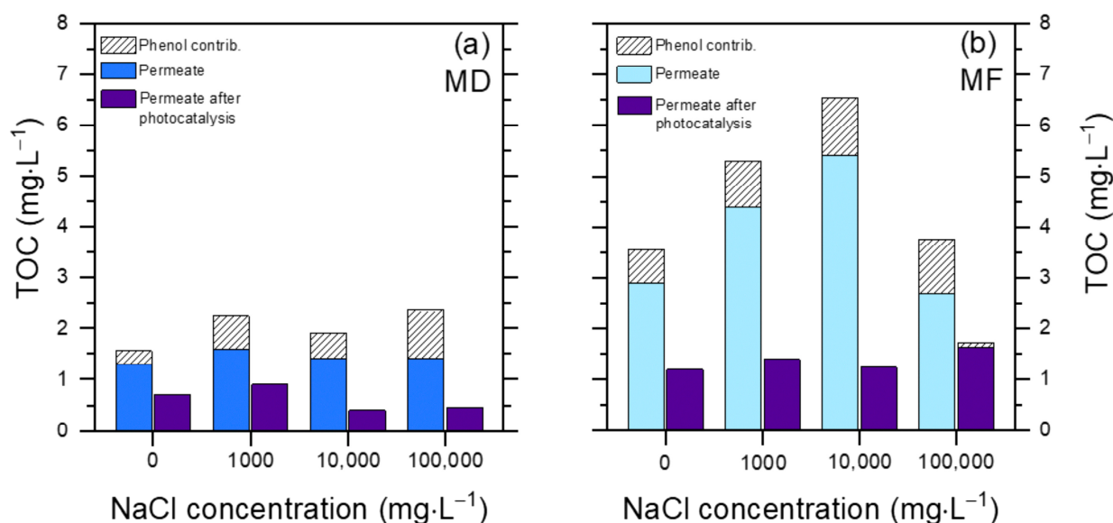
Figure 6. TOC removal from the PW permeate, upon UV-A irradiation in the presence of 0.5 g L -1 \text{TiO}_2 after 60 min. (a) MD permeate; (b) MF permeate. The contribution of phenol to the TOC value of the permeate solution before and after photocatalytic degradation is highlighted (in the latter case, it was the TOC value accounted for by the residual phenol that still occurred in the solution).
