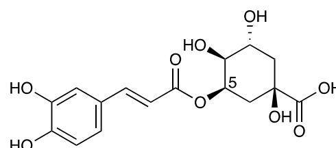
5-caffeoylquinic acid (1)
