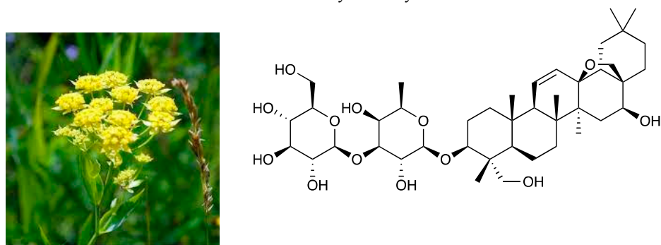
Saikosaponin A (58)
