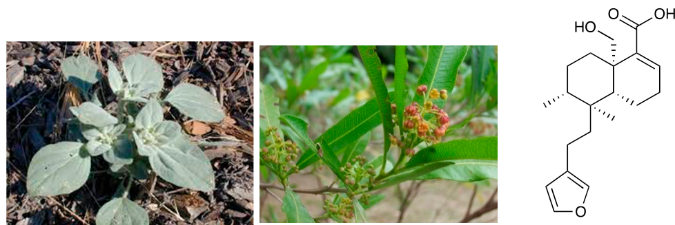
Hautriwaic acid (12)
