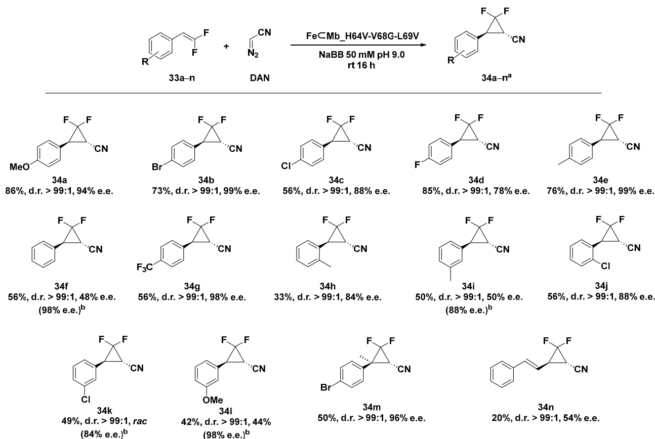
Scheme 11. Reaction conditions: reactions were carried out using 5 mM olefin 33a–n , 20 mM DAN, \text{FeC Mb\_H64V-V68G-L69V} expressing E. coli in 50 mM NaBB (sodium borate buffer) pH 9.0, rt 16 h, anaerobic conditions. [a] Yield as determined by fluorine NMR in presence of trifluorotoluene as internal standard. [b] e.e. obtained using \text{FeC Mb\_H64A-V68G-L69V} mutant [125].
