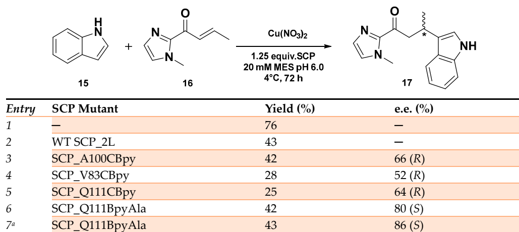
Scheme 7. Reaction conditions: reactions were carried out using 9 mol% of \text{Cu}(\text{NO}_3)_2 (90 \mu\text{M} ), SCP mutant (112.5 \mu\text{M} ), 1 mM of 15 and 2.5 mM of 16 in MES buffer (20 mM, 150 mM NaCl, pH 6.0) for 3 days at 4 °C. [a] reaction was conducted in MES buffer 20 mM, 150 mM NaCl, pH = 5.0 [94].
