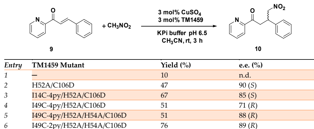
Scheme 4. Reaction conditions: reactions were carried out using TM1459 0.3 mM, CuSO 4 0.3 mM, substrate 9 10 mM, CH 3 NO 2 100 equiv., KPi (potassium phosphate buffer) pH 6.5/CH 3 CN 9:1, rt, 3 h [64].
