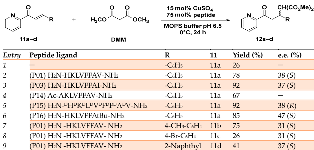
Scheme 5. Reaction conditions: reactions were carried out using 475 \mu M of peptide, CuSO 4 95 \mu M in 20 mM MOPS buffer pH 6.5, 0 ^{\circ} C, 24 h [72].
