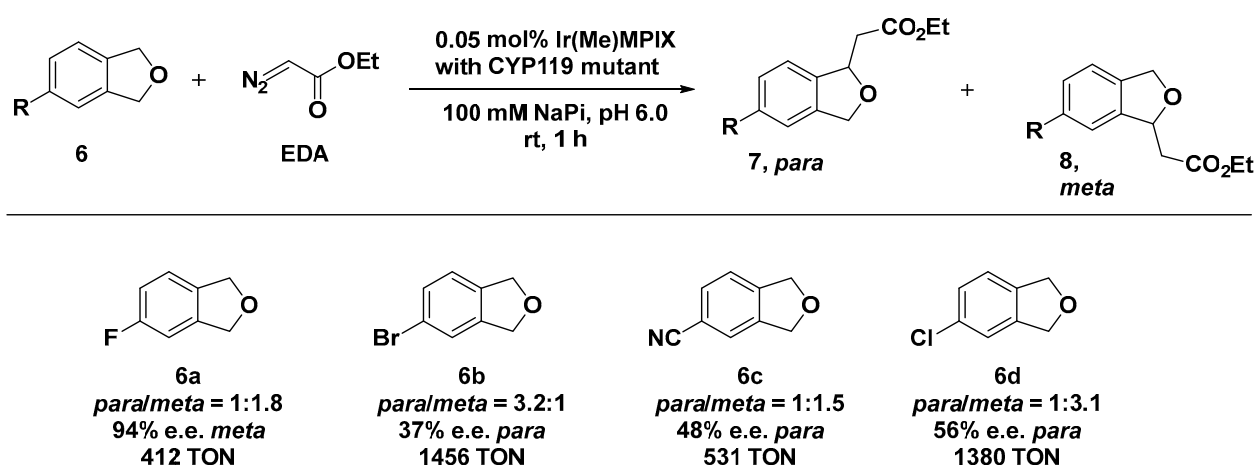
Scheme 3. Reaction conditions: reactions were carried out using 5mM of 6, 0.05 mol% of Ir(Me)MPIX<CYP119 MG 1 (6a) or Ir(Me)MPIX<CYP119 PG 2 (6b, 6c, and 6d), 100 mM NaPi (sodium phosphate buffer) pH 6.0, rt, 1 h [58].
