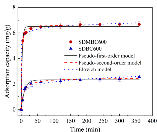
Figure 2. The adsorption kinetics of diuron by SDBC600 and SDMBC600 (5 mg/L diuron, 0.075 g SDMBC600, t = 0 –360 min).
