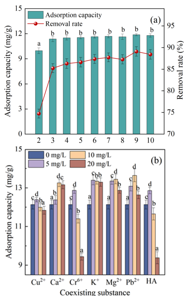
Figure 5. Effects of initial solution pH and coexisting substances on the adsorption of diuron by SDMB600: (a) initial solution pH; (b) coexisting substances. (10 mg/L diuron, 0.075 g SDMB600, t = 360 min). Different letters indicate significant differences between different treatments at the 0.05 level, testing by one-way ANOVA.
