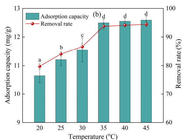
Figure 4. Effects of initial diuron concentration and solution temperature on the adsorption of diuron by SDMBC600: (a) initial diuron concentration; (b) solution temperature. (0.075 g SDMBC600, t = 360 min). Different letters indicate significant differences between different treatments at the 0.05 level, testing by one-way ANOVA.
