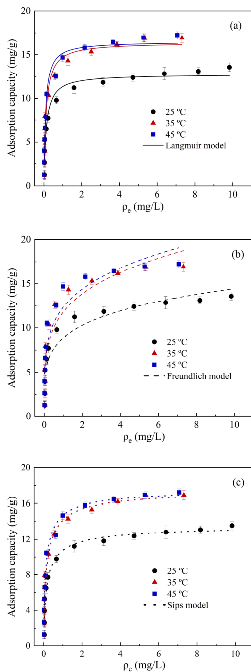
Figure 3. Isotherm model fitting of diuron adsorption by SDMBC600: (a) Langmuir model; (b) Freundlich model; (c) Sips model.
