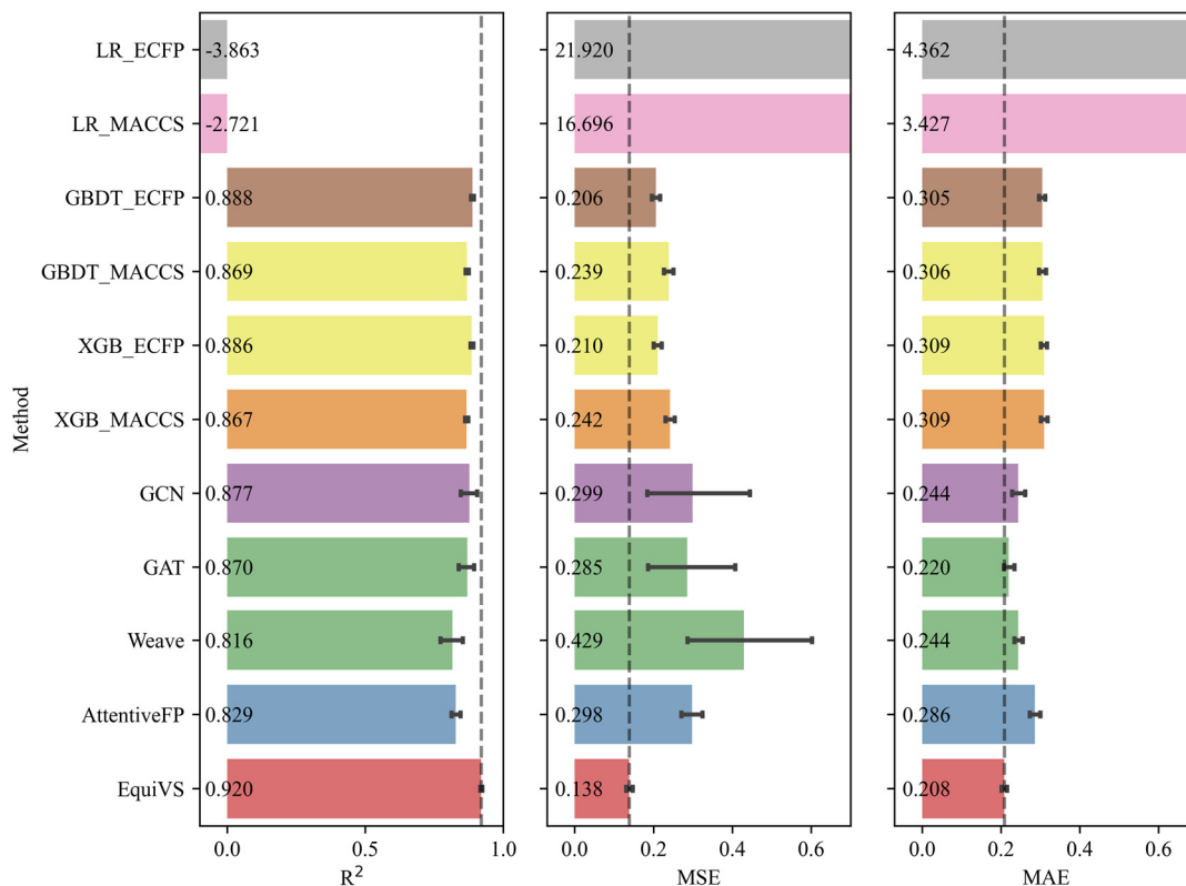
Figure 3. Model performances ( R^2 , MSE, and MAE) of EquiVS and 10 baseline methods on the bioactivity benchmark dataset of feasible targets.
