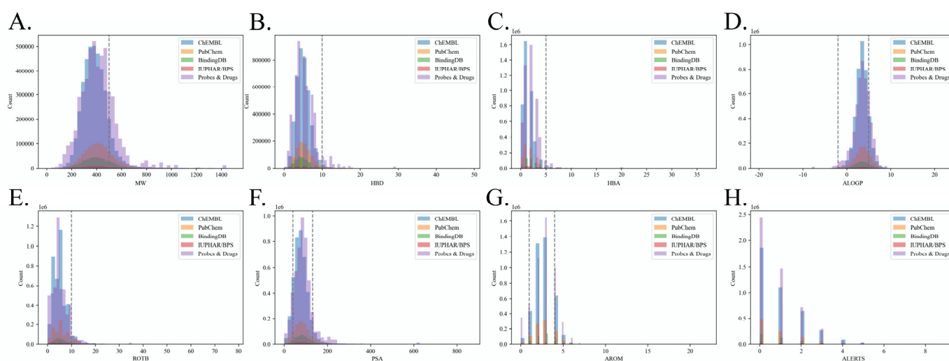
Figure 2. QED property distributions of benchmark dataset. (A) Distribution of MW; (B) Distribution of Num. HBD; (C) Distribution of Num. HBA; (D) Distribution of AlogP; (E) Distribution of Num. ROTB; (F) Distribution of PSA; (G) Distribution of Num. AROM; (H) Distribution of Num. ALERTS.
