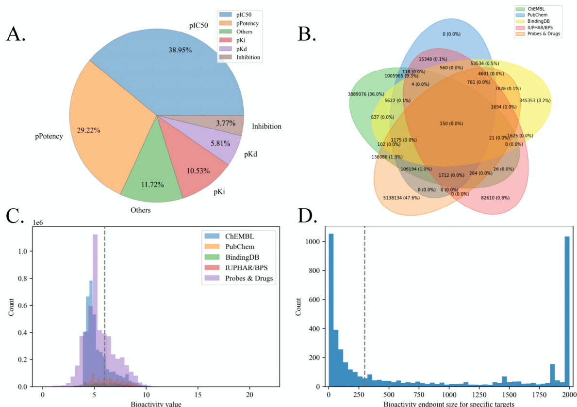
Figure 1. Distribution visualization of raw bioactivity endpoints. A. Pie plot of bioactivity type proportion.
