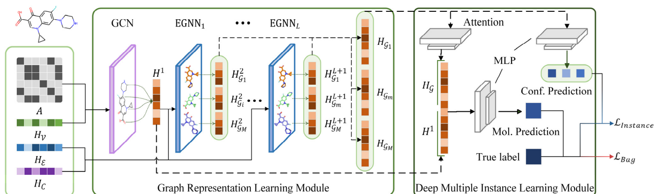
Figure 8. The architecture of EquiVS.
