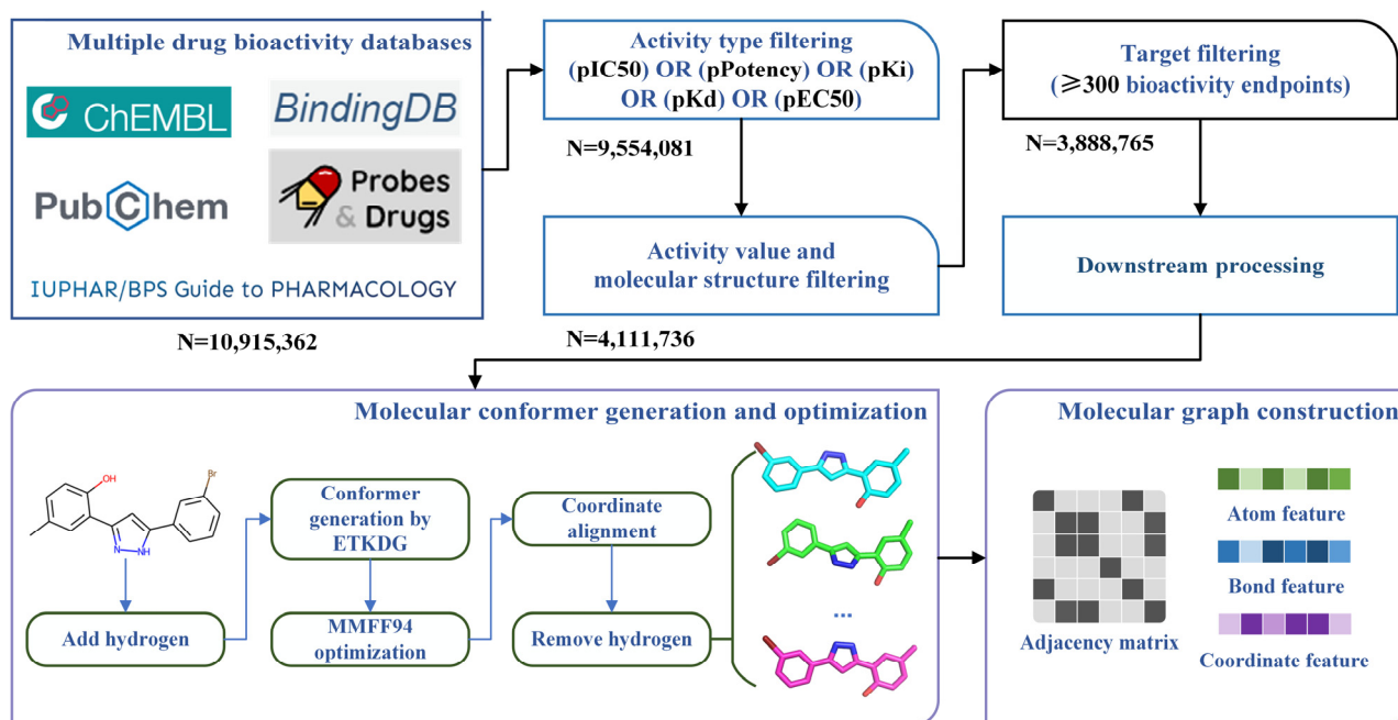
Figure 6. Bioactivity data collecting, integrating, filtering and processing workflow.
