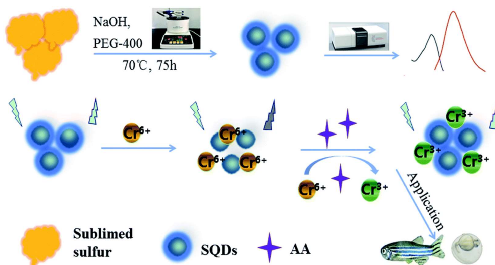
Figure 7. Schematic illustration of the SQDs-based “ON–OFF–ON” fluorescence sensor. Adapted from ref. [55] Copyright 2021 Royal Society of Chemistry.
