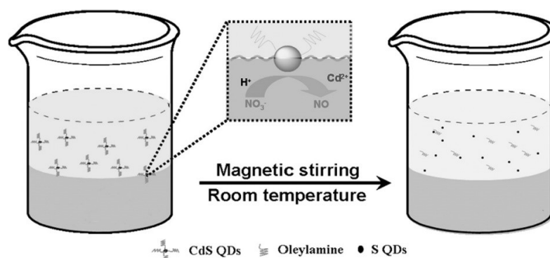
Figure 1. Schematic illustration of the synthesis of SQDs from CdS QDs. Adapted from ref. [19] Copyright 2014 Wiley.
