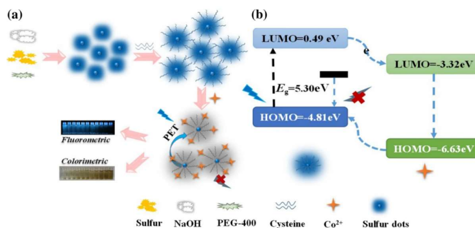
Figure 8. (a) Schematic representations of cysteine-modified SQDs are used for fluorescence and colorimetric dual-channel detection of \text{Co}^{2+} ; (b) Fluorescence quenching process of cysteine-modified SQDs toward \text{Co}^{2+} through photoinduced electron transfer. Adapted from ref. [62]. Copyright 2020 Springer.
