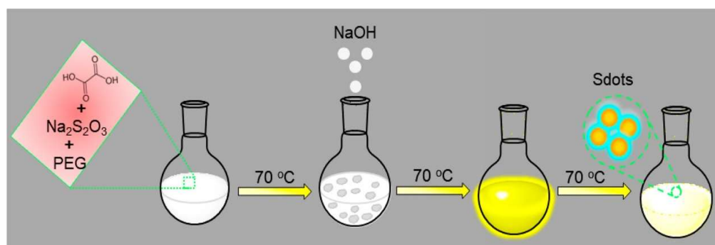
Figure 6. Schematic representation of the synthesis of SQDs. Adapted from ref. [42] Copyright 2020 American Chemical Society.
