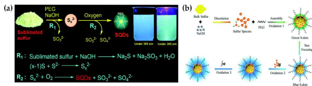
Figure 4. (a) Proposed formation mechanism of SQDs under \text{O}_2 atmosphere. Adapted from ref. [32] 2020 Royal Society of Chemistry; (b) schematic illustration of the synthesis and the PL mechanisms of S-dots. Adapted from ref. [33] 2022 Royal Society of Chemistry.
