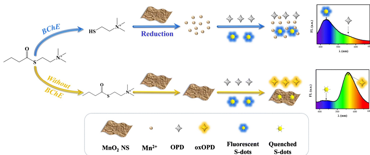
Figure 9. Schematic illustration of the ratiometric fluorescence assay for detection of BChE activity. Adapted from ref. [21] Copyright 2021 Springer.
