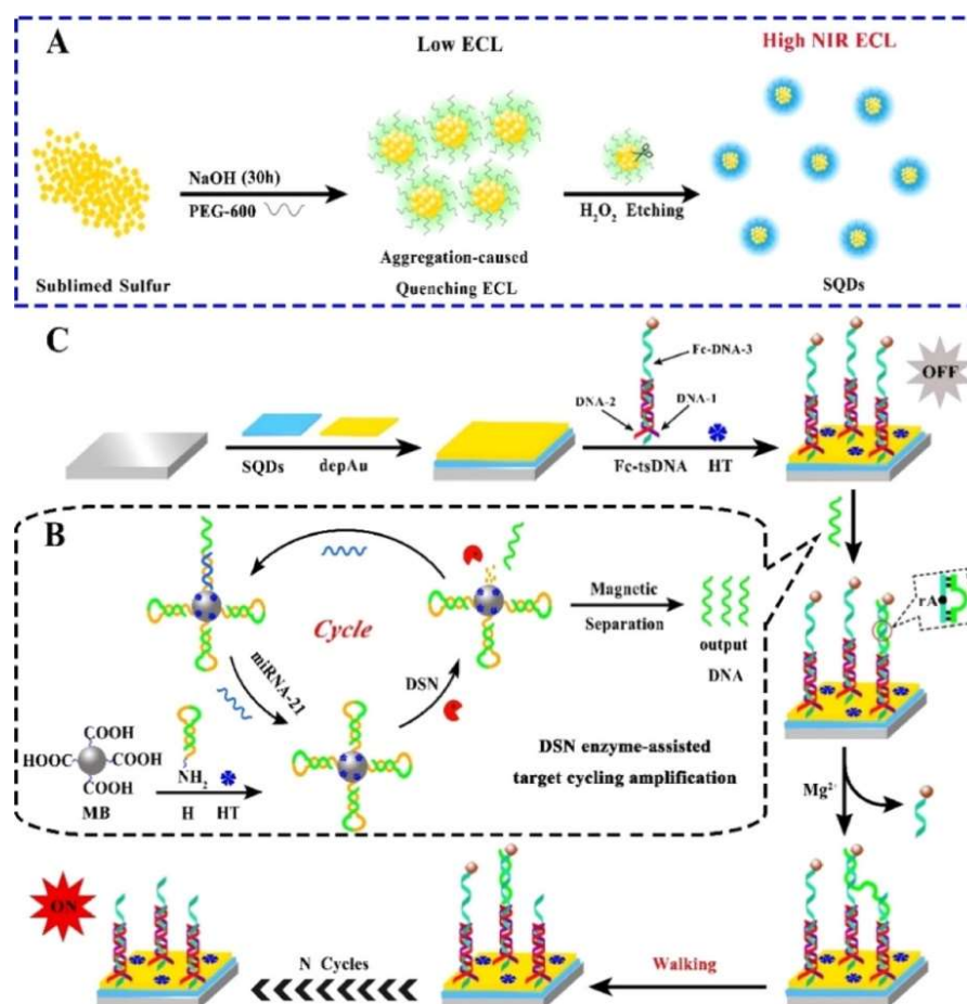
Figure 11. SQDs as a biosensor in ECL and detection of DNA. (A) Schematic diagram of the preparation of SQDs, (B) Schematic illustration of miRNA-21 detection, and (C) Modification of the electrode. Adapted from ref. [75] Copyright 2020 American Chemical Society.
