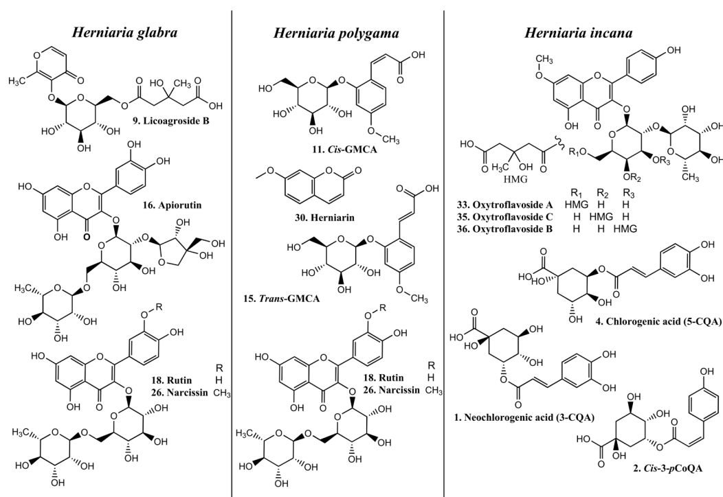
Figure 1. Chemical structures of the main phenolic metabolites in the studied Herniaria purified extracts.
