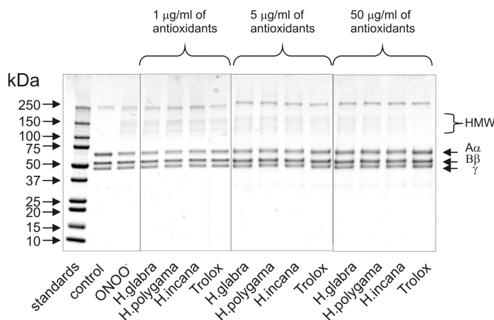
Figure 4. Protective effects of the examined Herniaria glabra , H. polygama and H. incana herb purified extracts on the ONOO − -induced oxidative changes in fibrinogen structure. The figure includes a representative SDS-PAGE pattern of human fibrinogen, obtained from the executed experiments employing 4–20% Mini-PROTEAN ® TGX ™ Precast Protein Gels and staining with Coomassie Brilliant Blue R-250 dye ( n = 3 ).
