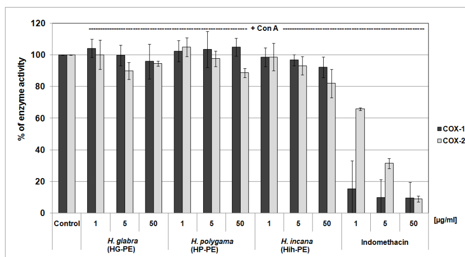
Figure 5. Screening of the cyclooxygenase-inhibitory properties of the examined Herniaria glabra (HG-PE), H. polygama (HP-PE), and H. incana herb (Hih-PE) purified extracts. The enzyme activity in control samples (untreated with the extracts or a reference inhibitor) was assumed as 100%; n = 3 .
