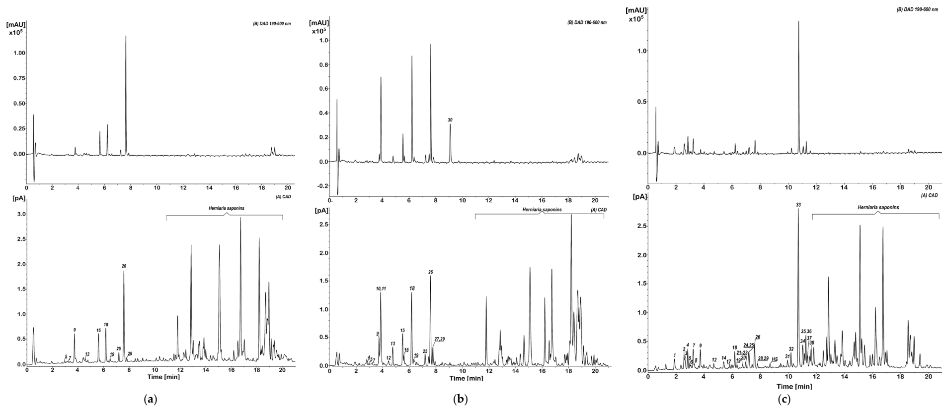
Figure 2. UHPLC—diode array detector (DAD) and charged aerosol detector (CAD) profiles of the purified extracts from (a) Herniaria glabra ; (b) H. polygama ; (c) H. incana herb.
