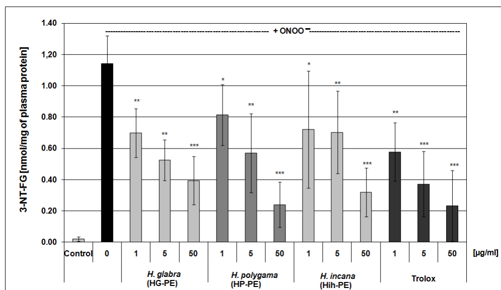
Figure 3. Protective effects of the examined Herniaria glabra (HG-PE), H. polygama (HP-PE) and H. incana herb (Hih-PE) purified extracts on the ONOO − -induced formation of 3-nitrotyrosine in blood plasma proteins. Human plasma was exposed to 100 µM ONOO − in the presence or absence of the tested extracts or a reference compound (Trolox); * p < 0.05 , ** p < 0.01 , *** p < 0.001 ; n = 6 .
