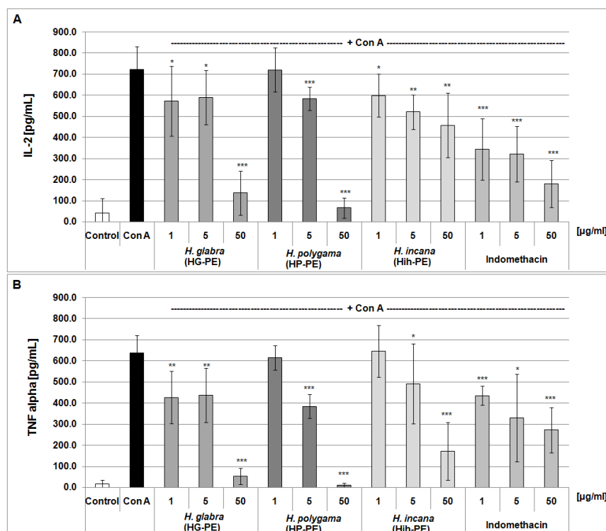
Figure 6. Effects of the examined Herniaria glabra (HG-PE), H. polygama (HP-PE) and H. incana herb (Hih-PE) purified extracts on the inflammatory response of the concanavalin A-stimulated human PBMCs. Anti-inflammatory actions of the tested extracts were estimated using ELISA and based on IL-2 (panel A) and TNF- \alpha (panel B) release; * p < 0.05 , ** p < 0.01 , *** p < 0.001 ; n = 4-5 .
