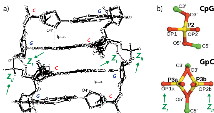
Figure 4. Z_I and Z_{II} conformations. (a) Superimposition of two Z-DNA d(\text{CGCG})_2 structures (PDBid: 1ZNA; resolution 1.5 Å) showing Z_I (light bonds) and Z_{II} (dark bonds) conformations (adapted with permission from [38]). Short \text{lp}\dots\pi contacts are marked by a dotted line. (b) Two characteristic conformations of a CpG (top) and a GpC (bottom) step extracted from a d(\text{CGCGCGCGCGCG})_2 dodecamer (PDBid: 4OCB; resolution: 0.75 Å). The CpG step displays mostly a single conformation while four of the five GpC steps of the dodecamer were modeled as alternate Z_I and Z_{II} conformations thanks to the use of phosphorous anomalous signals (adapted from [34]).
