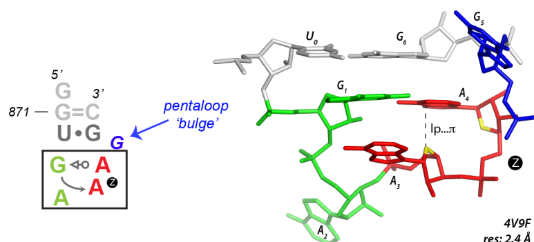
Figure 7. An r(G 1 AAAg) pentaloop that adopts a Z-turn rather than an expected U-turn. The Z-step is marked by a circled “Z” in both the secondary and tertiary structure of the ribosomal H35a tetraloop of the Haloarcula marismortui large ribosomal subunit (PDBid: 4V9F). This motif is conserved in all known ribosome structures. It can be considered as a “shapeshifting” motif exemplifying the ability of an r(GAAA) loop to switch from U-turns to Z-turns in specific environments [13,31]. Note that a U-turn is characterized by an sOP2 phosphate... \pi contact between the first and third residue (not shown), while Z-turns are characterized by sO4'3 between the 3rd and 4th residue and Z anti -turns by sO4'5 between the 3rd and 4th residue (Figure S5).
