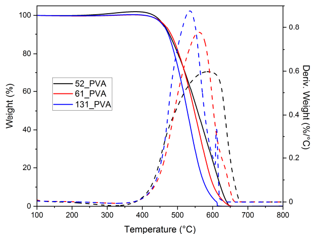
Figure 2. TG (solid) and DTG (dashed) curves recorded in flowing air for the carbon materials of various grain sizes synthesized by the carbonization of PVA-stabilized resol resins at 600 °C.
