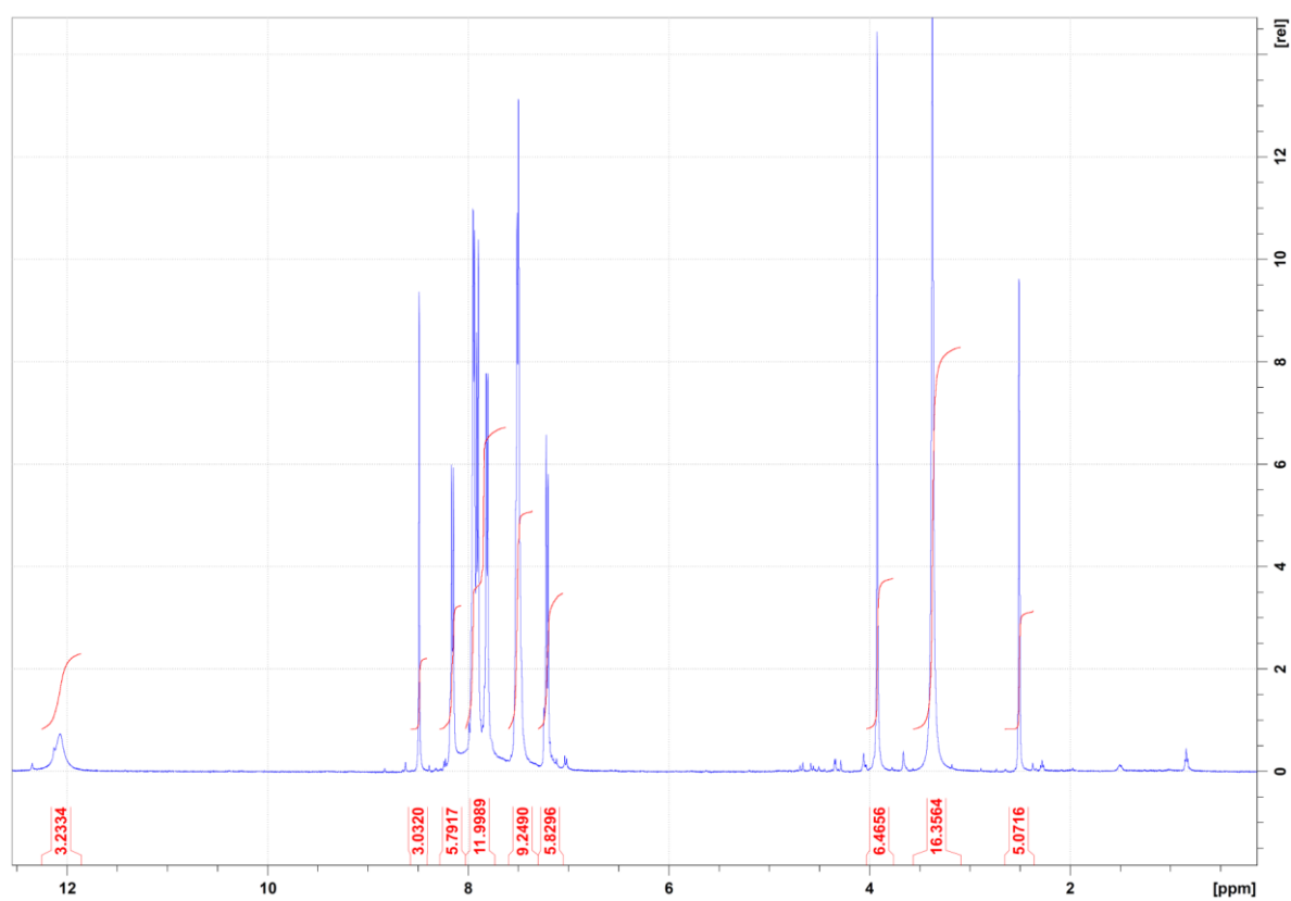
Figure 3. 1 H-NMR spectrum of Compound 6a.
