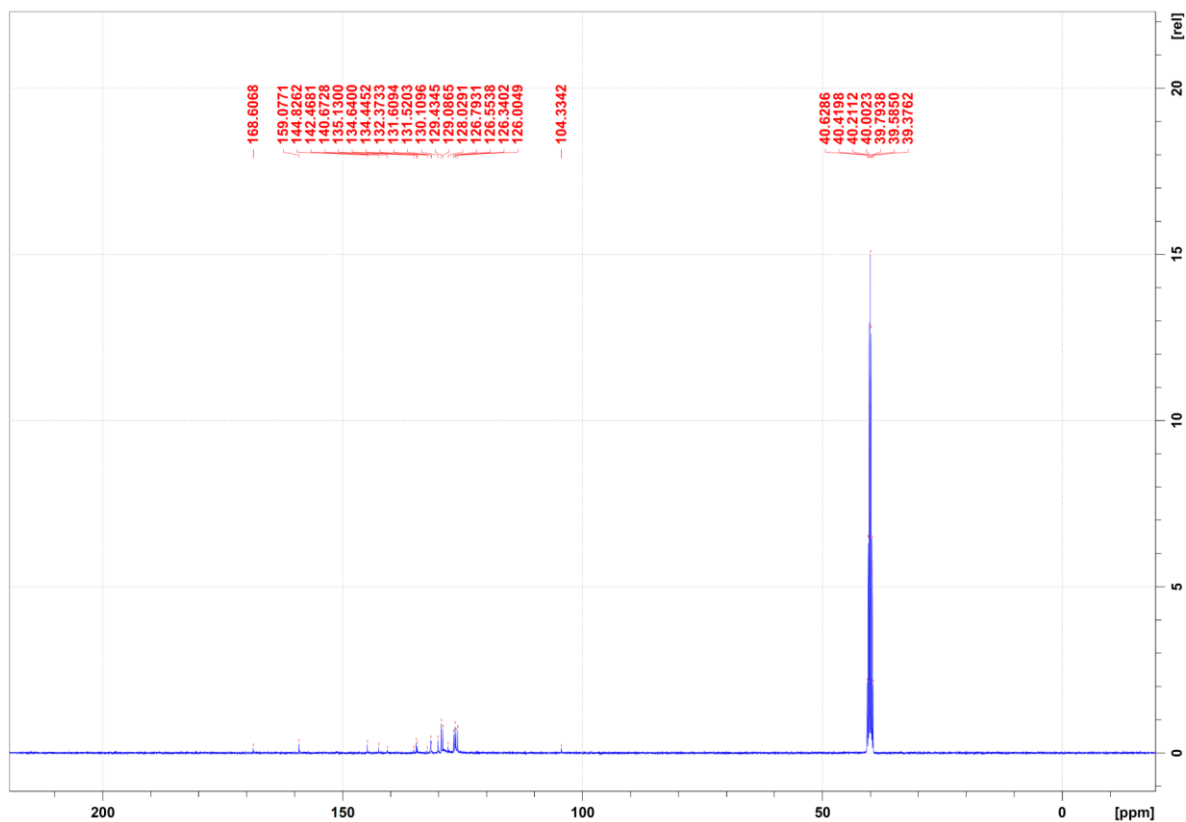
Figure 10. 13 C-NMR spectrum of Compound 9a.
