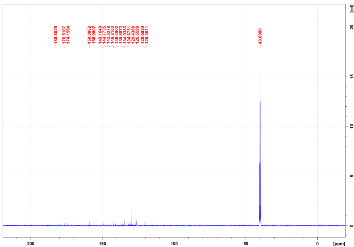
Figure 20. 13 C-NMR spectrum of Compound 16a.
