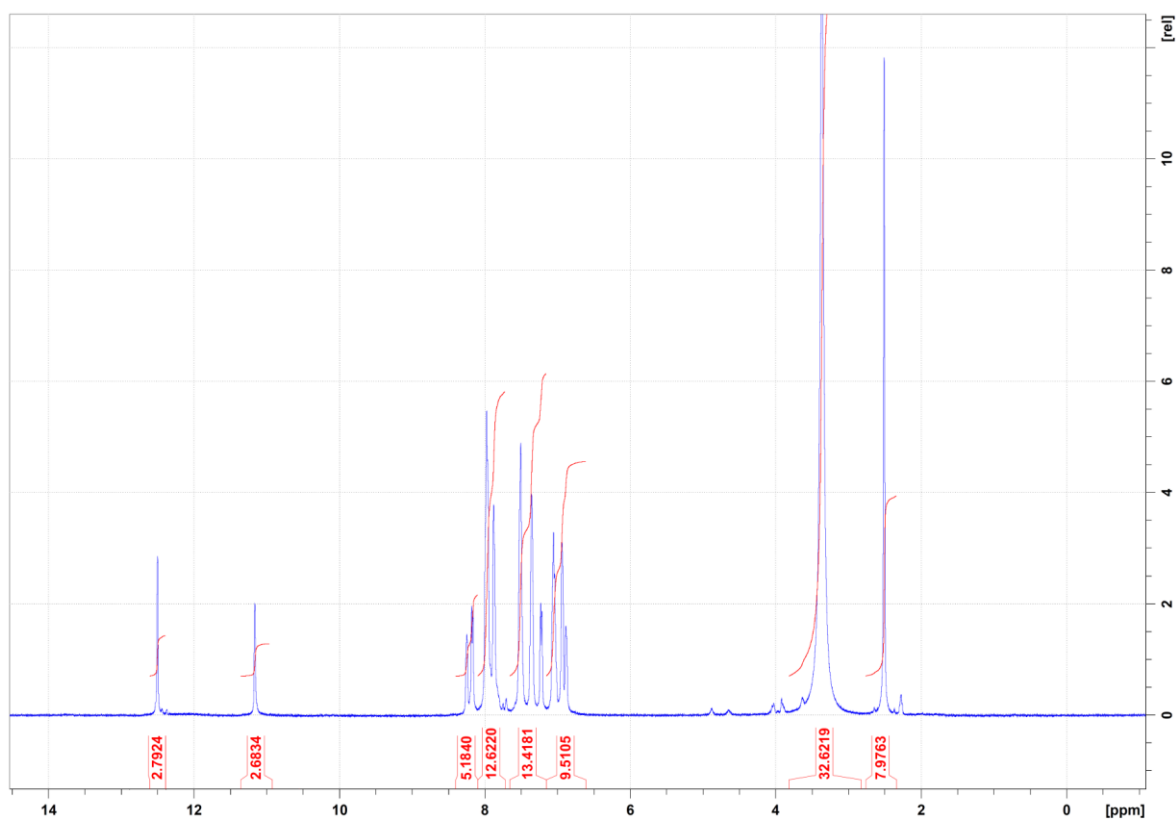
Figure 17. 1 H-NMR spectrum of Compound 12.
