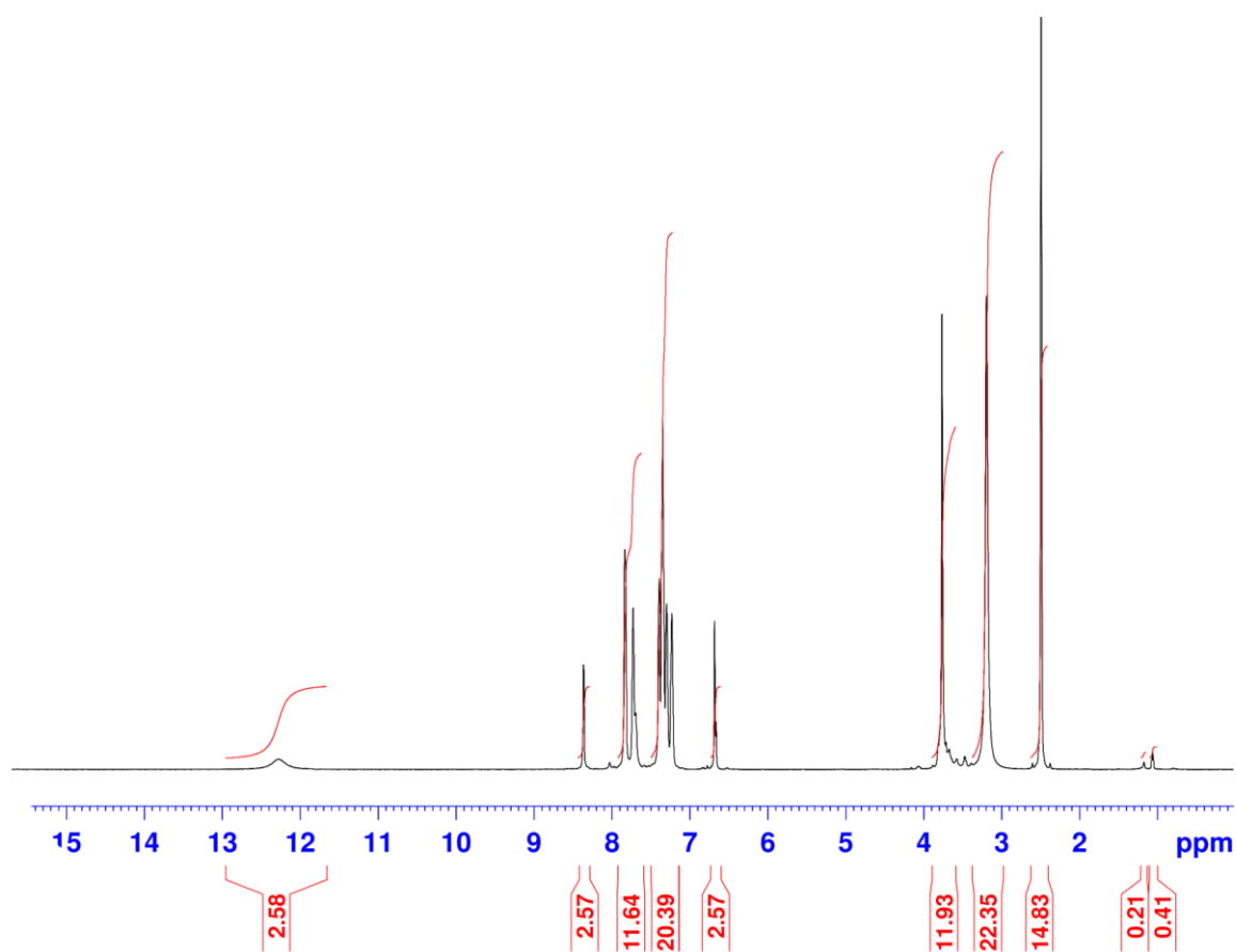
Figure 13. ^1\text{H} -NMR spectrum of Compound 10.
