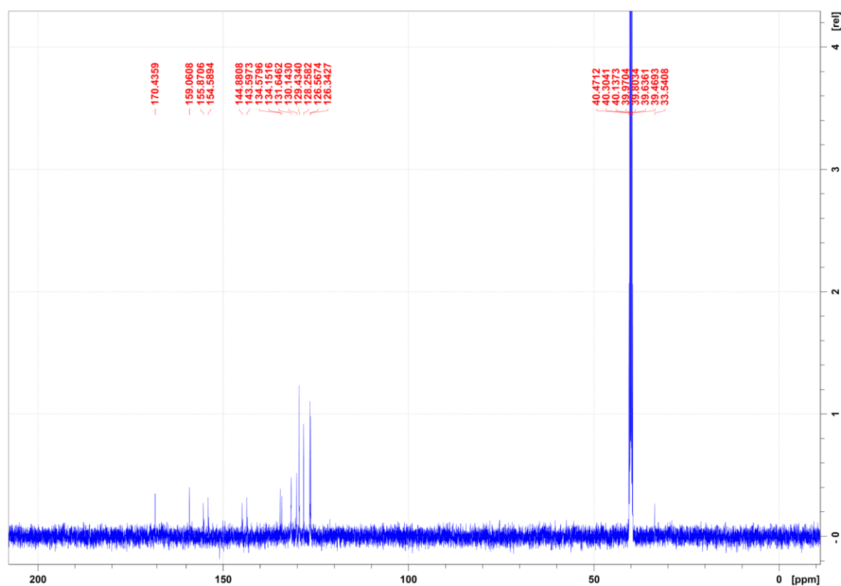
Figure 4. ^{13}\text{C} -NMR spectrum of Compound 6a.
