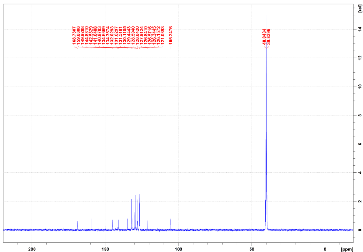
Figure 12. ^{13}\text{C} -NMR spectrum of Compound 9b.
