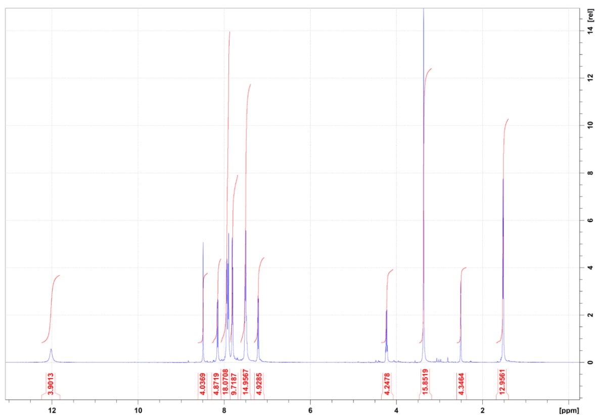
Figure 5. ^1\text{H} -NMR spectrum of Compound 6b.
