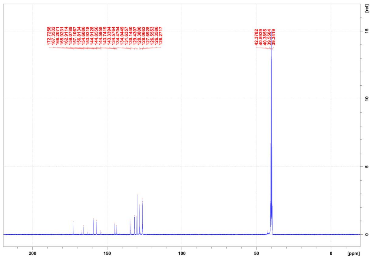
Figure 16. 13 C-NMR spectrum of Compound 11.
