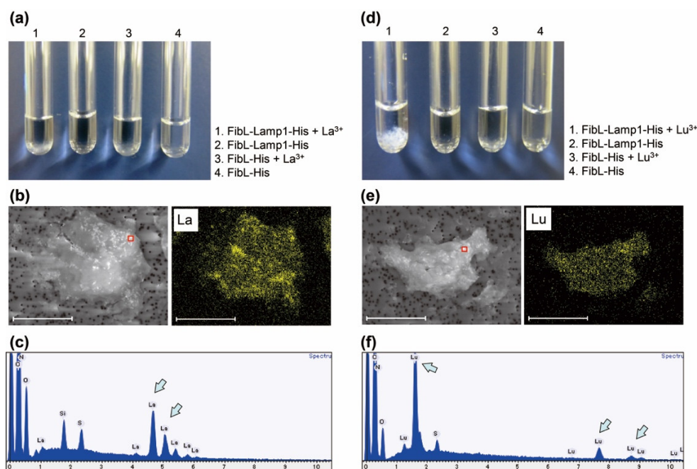
Figure 3. \text{La}^{3+} and \text{Lu}^{3+} recognition with the purified FibL-Lamp1-His protein. (a–c) Reaction with \text{La}^{3+} , and (d–f) reaction with \text{Lu}^{3+} . (a–d) Optical image of precipitation induced by the purified FibL-Lamp1-His protein. (b–e) SEM image (left) and elemental mapping image (right) of precipitation. Scale bars, 100 \mu\text{m} . (c–f) EDX spectrum. The red frame area in the SEM image was analyzed. Each arrow indicates the spectrum of La or Lu.
