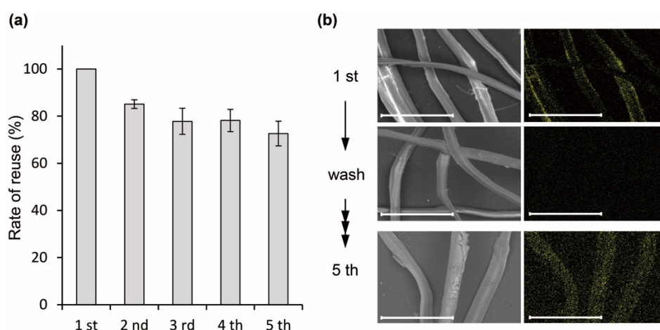
Figure 7. Reusability of silk powder for Dy^{3+} recovery. (a) The relative degree to the initial Dy^{3+} recovery efficiency is shown. Averages and standard deviations for three independent experiments were represented. (b) SEM-EDX analysis, the captured Dy (yellow signal) was eluted with acetic buffer (50 mM) at pH 4.0, and the silk powder was recycled. Scale bars: 100 \mu m .
