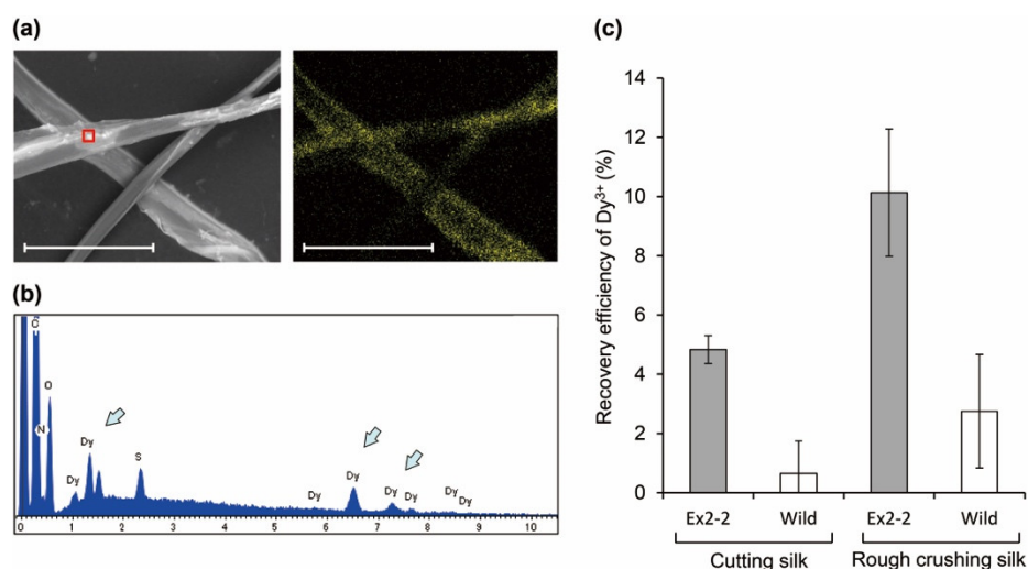
Figure 6. Dy^{3+} recognition with silk powder: (a) SEM (left) and elemental mapping (right) images of silk powder after Dy^{3+} absorption reaction. The yellow signal indicates a Dy. Scale bar, 80 \mu m , (b) EDX spectrum, each arrow indicates the Dy signal and (c) the recovery efficiency of Dy^{3+} of silk with harvested silk from Ex2-2. Averages and standard deviations for three independent experiments were represented.
