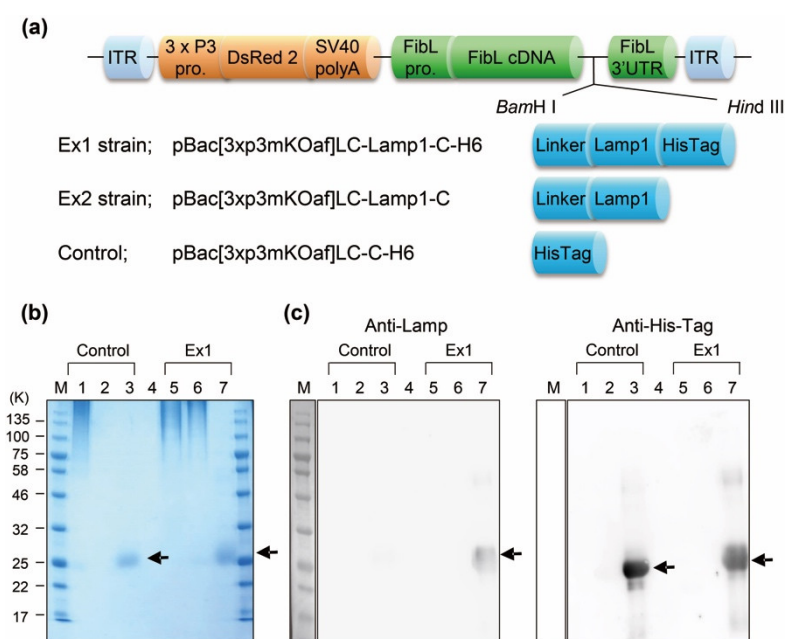
Figure 1. Breeding of the transgenic silkworm. (a) Construction of the expression vector. Each plasmid contains expression units for selection marker gene ( DsRed2 ) and cDNA of fibroin L-chain ( FibL cDNA) between the piggyBac inverted terminal repeat (ITR). Three gene fragments containing Lamp1 or His Tag were inserted into the 3' ends of FibL cDNA using restriction site of Bam H I and Hind III. 3xP3 pro., 3xP3 promoter; SV40 polyA, polyA signal of SV40; FibLpro., promoter of fibroin L-chain; and FibL 3' UTR, 3' untranslated region of fibroin L-chain. (b) SDS-PAGE analysis of purified FibL-Lamp1-His protein from Ex1 strain and the control strain. (c) Western blotting analysis using Lamp1, and His-tag antibody. Each arrow indicates the expected molecular weight of the target protein. Lane 1, FibL sample before purification; Lane 2, flow-through of FibL column; Lane 3, purified FibL; Lane 4, buffer; Lane 5, FibL-Lamp1 sample before purification; Lane 6, flow-through of FibL-Lamp1 column; and Lane 7, purified FibL-Lamp1.
