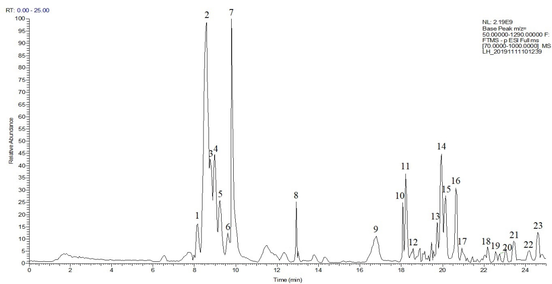
The total ion current of CFP identified by UHPLC-HESI-MS/MS
