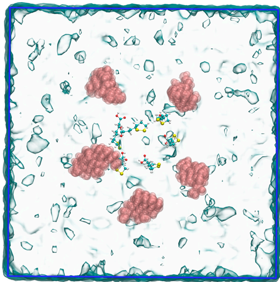
Figure S1. The initial model of ALAs (ball-and-stick model) and chitosan hexamers (vdW surface model) in water box.
