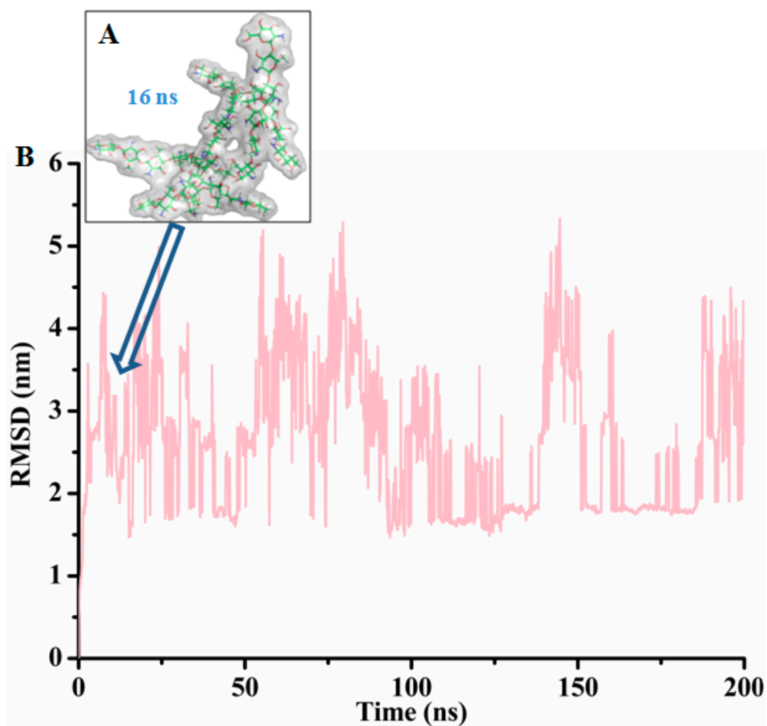
Figure S2. RMSD analysis. (A) The chitosan micelle model formed after 16 ns simulation time, (B) The RMSD curve of chitosan.
