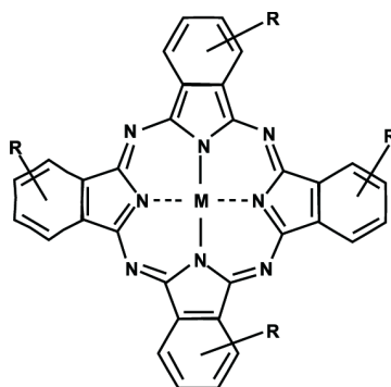
Scheme 1. General structure of the phthalocyanine macrocycle, where M is the central metal ion or \text{H}_2 in the case of the free base. R is the potential functionalization on the phthalocyanine periphery.
