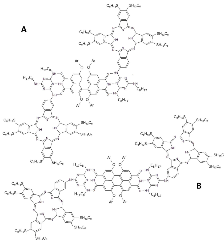
Figure 5. Melanine substituted Pc used to form the supramolecular assembly with functionalized PDI derivative [71]. In (A) and (B) the two possible supramolecular configurations are reported according to the authors' rationale [71].
