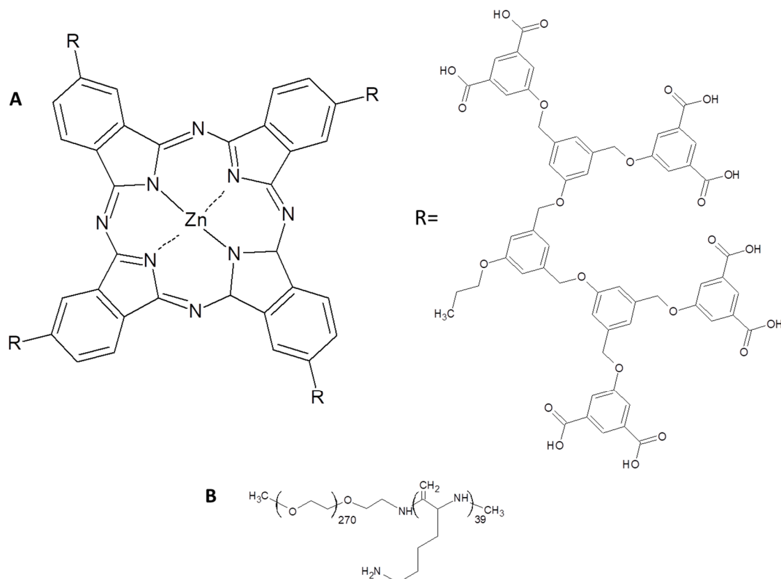
Figure 31. (A) dendrimeric ZnPc; (B) PEG–PLL used in [171].
