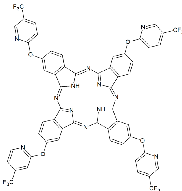
Figure 35. Chemical structure of the free base 4-((5-(trifluoromethyl)pyridin-2-yl)oxy)phthalocyanine utilized to assemble the hybrid structures with GQDs in the ref. [191].
