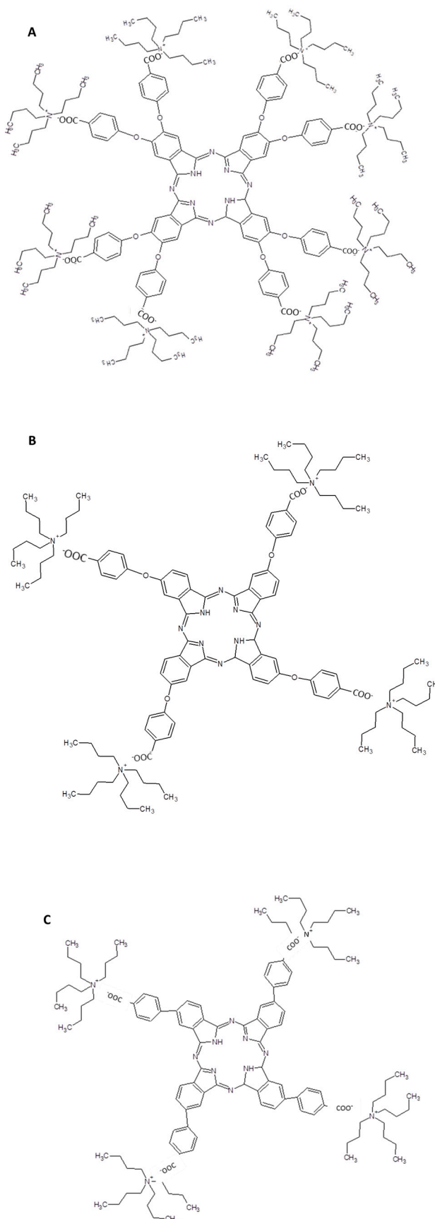
Figure 9. Chemical structures of the three carboxylated phthalocyanines used to form the electrostatically bounded supramolecular dyads with \text{Li}^+\text{@C}_{60} [84]. A , B and C are the three phthalocyanine derivatives used to form complexes with fullerenes.
