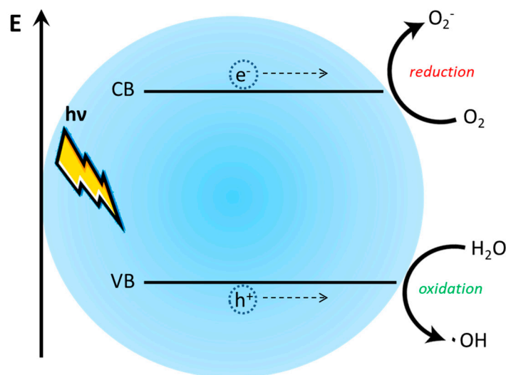
Figure 22. Schematization of the photo-induced formation of the radical \text{O}_2^{\bullet-} and the formation of the hydroxyl radical ( \text{OH}^{\bullet} ).
