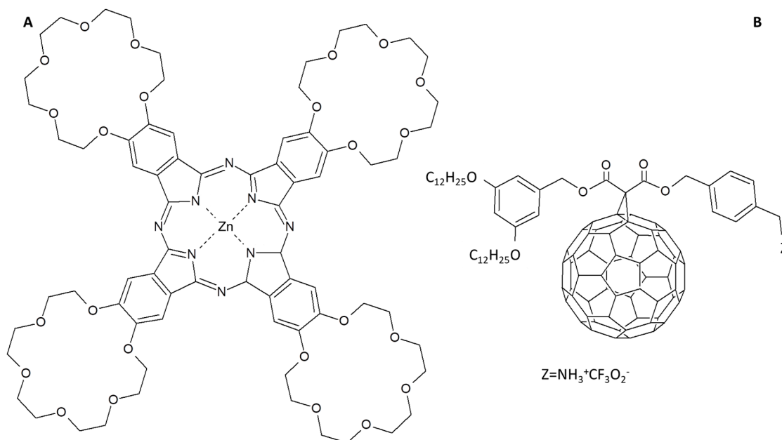
Figure 10. (A) 18-crown tetra functionalized ZnPc and (B) C_{60} derivative chemical structures [85].
