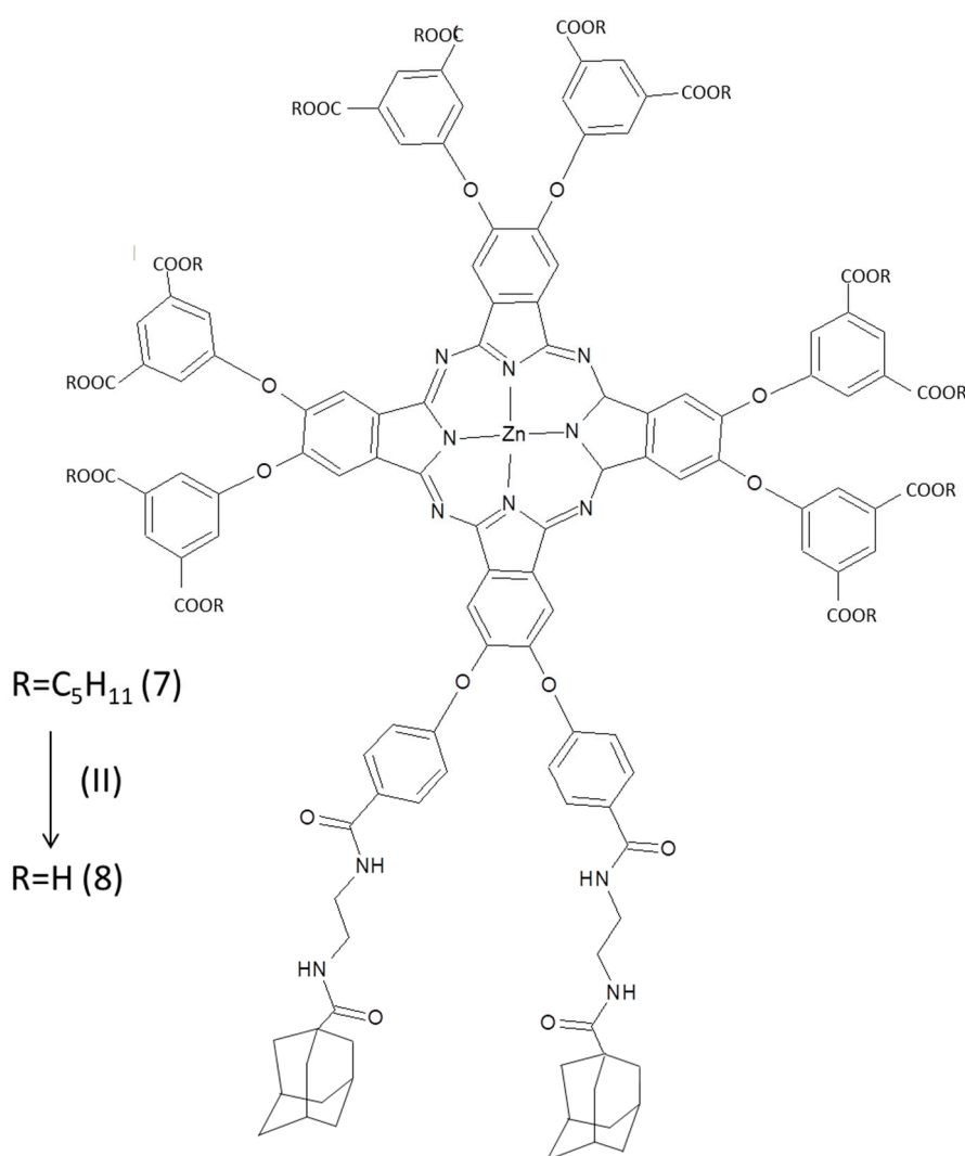
Figure 26. Octahoxosubstituted ZnPc bearing two adamantane groups [140].
