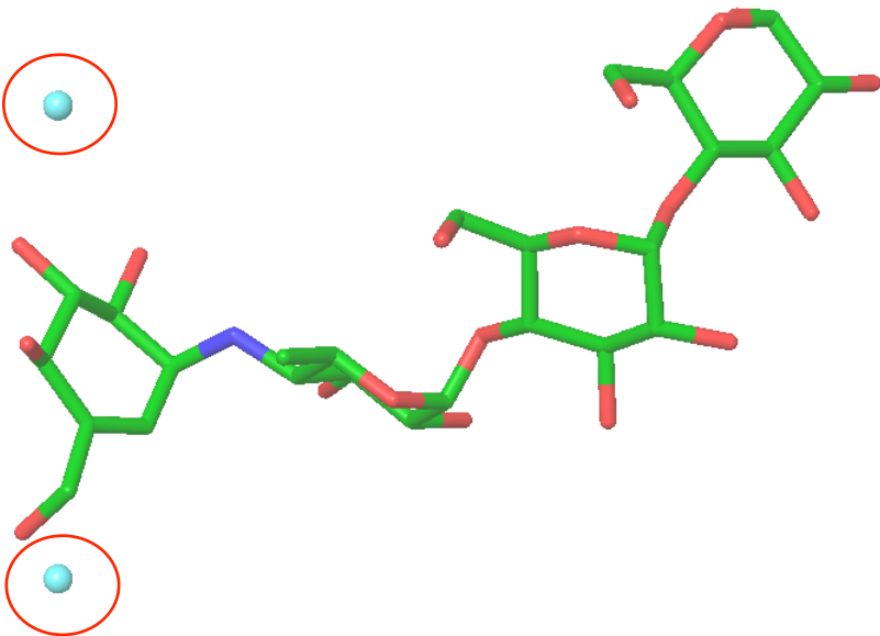
acarbose
