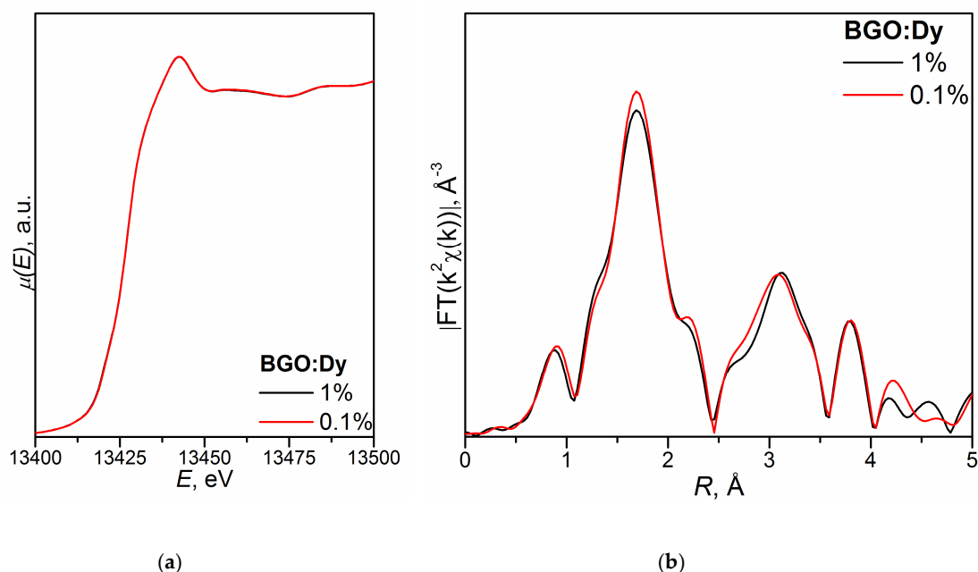
Figure 9. Bi L 3 -edge (a) XANES spectra and (b) EXAFS Fourier transforms ( k -range, 2–13 \text{\AA}^{-1} ) for the BGO:1.0Dy and BGO:0.1Dy samples.
