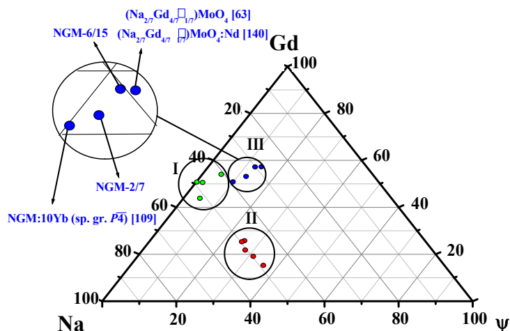
Figure 3. Region of existence of phases with the general composition (\text{Na}, \text{Gd}, \psi)\text{MoO}_4 with \psi = 0 , \square (vacancy), Yb, La. Region III with defective and ordered structures is highlighted.
