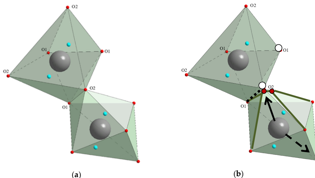
Figure 10. Model of rearrangement of (a) the BiO 6 and DyO 6 octahedra into (b) the vacancy BiO 5 octahedron and DyO 7 octahedron with a split top. The solid arrow shows the direction of Dy 3+ displacement with the formation of the DyO 7 polyhedron. The dashed arrow shows the direction of Dy 3+ displacement o with the formation of the DyO 5 polyhedron.
