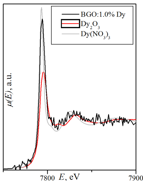
Figure 11. Dy L 3 -edge XANES data for the BGO:1.0Dy and reference samples: Dy 2 O 3 and Dy(NO 3 ) 3 .
