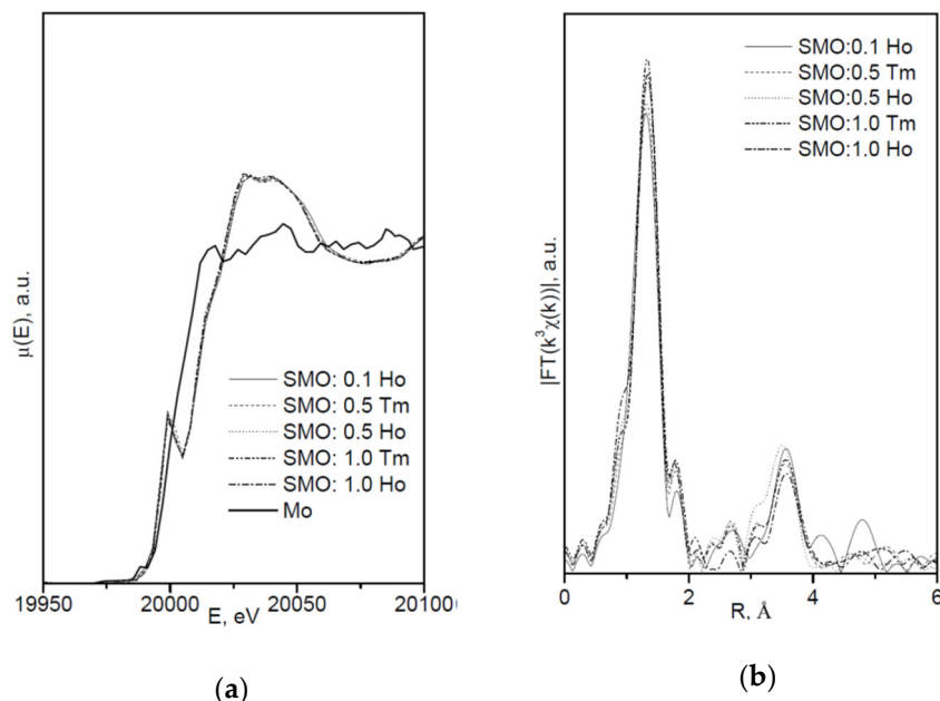
Figure 2. Mo K-edge-normalized (a) X-ray absorption spectroscopy (XANES) spectra and (b) EXAFS Fourier transforms for SrMoO 4 :Ho and SrMoO 4 :Tm crystals. The standard is metal molybdenum.
