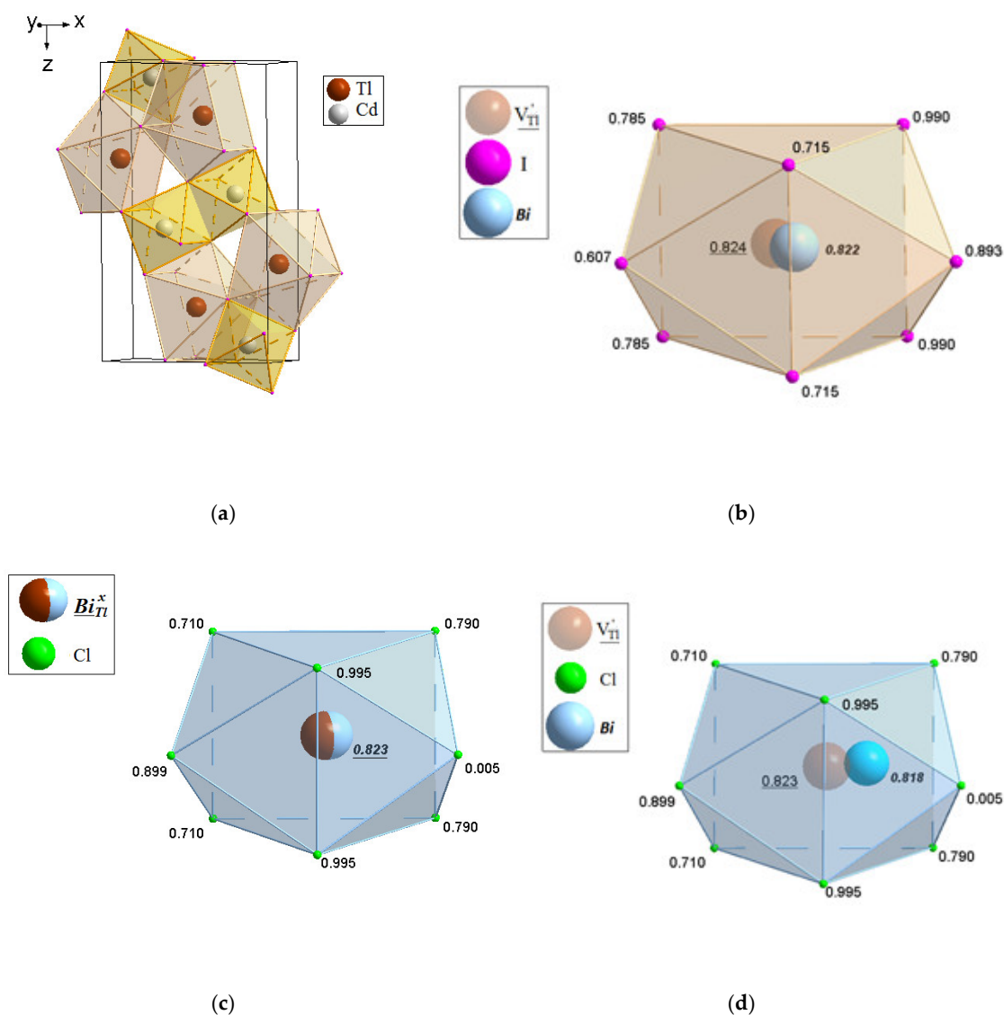
Figure 16. (a) Structure of TlCdX 3 (X = Cl, I); (b) The (Tl,Bi)I 3 , (c) (Tl,Bi)Cl 3 , (d) (Tl,Bi)Cl 3 coordination polyhedra.
