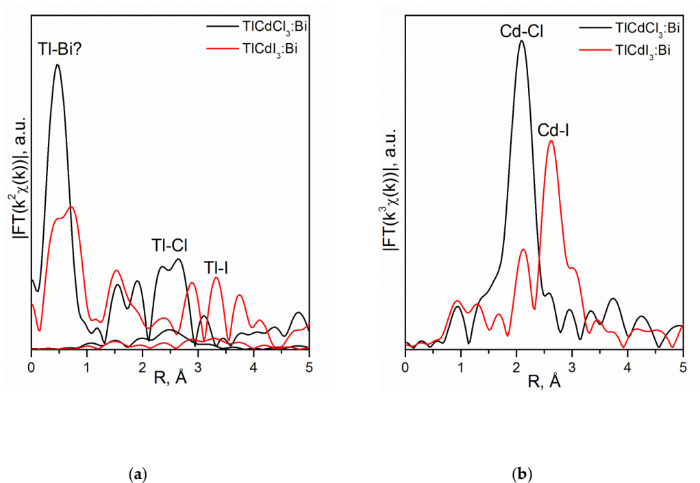
Figure 18. EXAFS Fourier transform curves measured (a) at the Tl L 3 -edge and (b) at the Cd K-edge for TlCdCl 3 :Bi and TlCdI 3 :Bi crystals.
