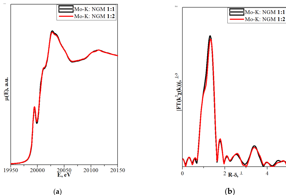
Figure 5. Mo K-edge-normalized (a) XANES spectra and (b) EXAFS Fourier transforms for NGM 1:1 (black curves) and NGM 1:2 (red curves) samples.
