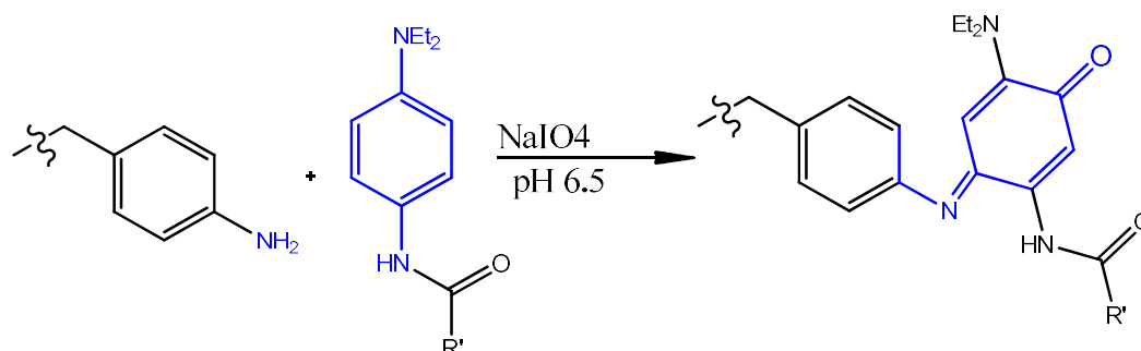
Figure 33. Oxidative coupling via a periodate-mediated reaction of phenylenediamine with aniline groups.
