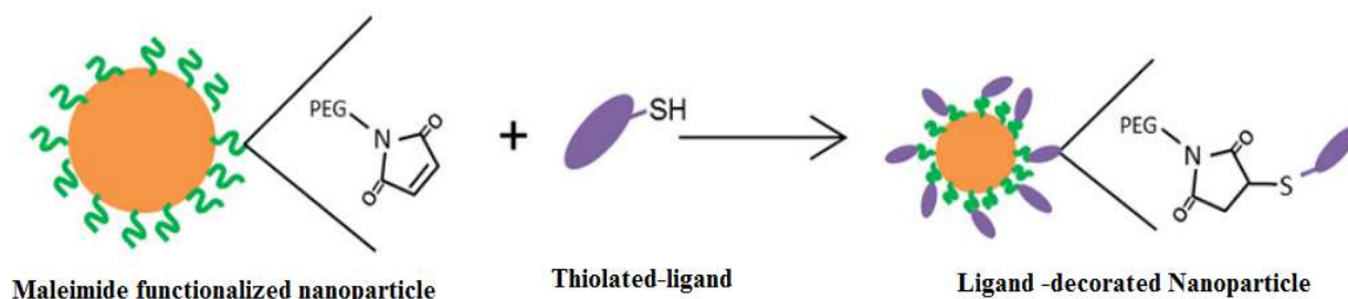
Figure 28. Thiol maleimide coupling chemistry [27].
