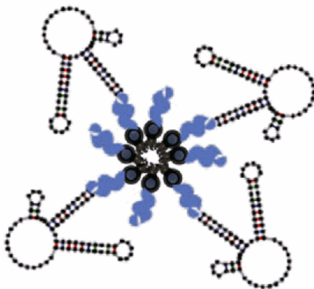
Figure 23. DSPE-PEG-Apt1 micelles. [49]
