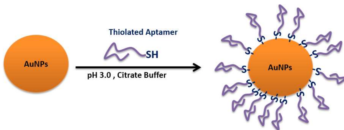
Figure 31. Coordination attachment of thiolated nucleic acids to gold nanoparticles (AuNPs).
