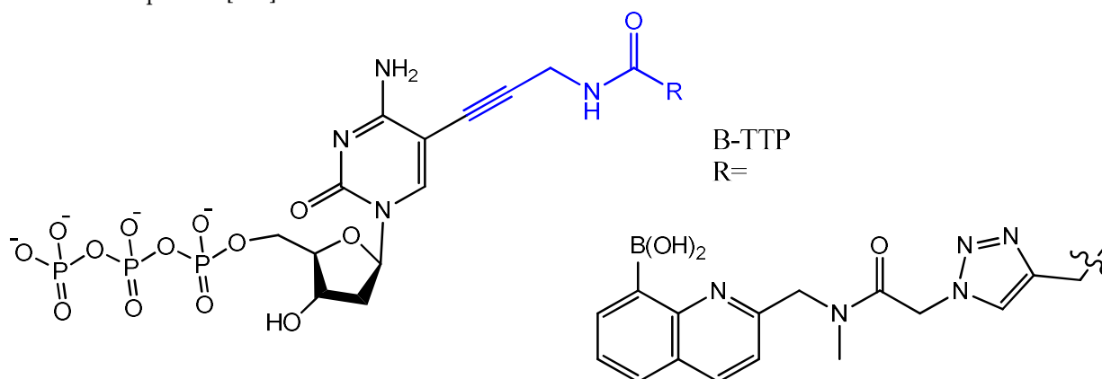
Figure 17. The chemical structures of B-TTP.
