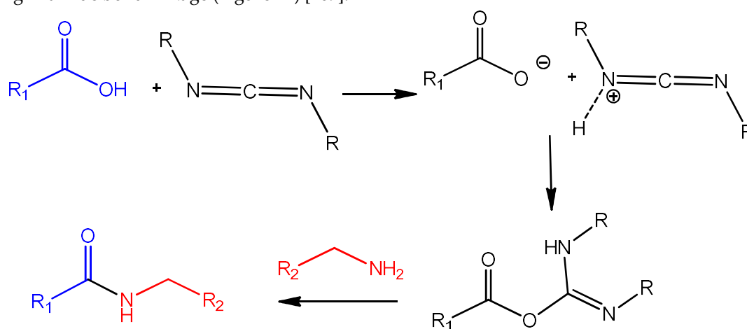
Figure 24. The formation of a covalent amide bond via carbodiimide coupling.
