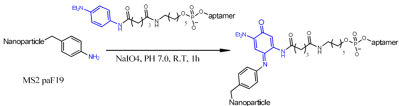
Figure 34. The MS2 surface was functionalized with sgc8c aptamer via oxidative coupling chemistry.
