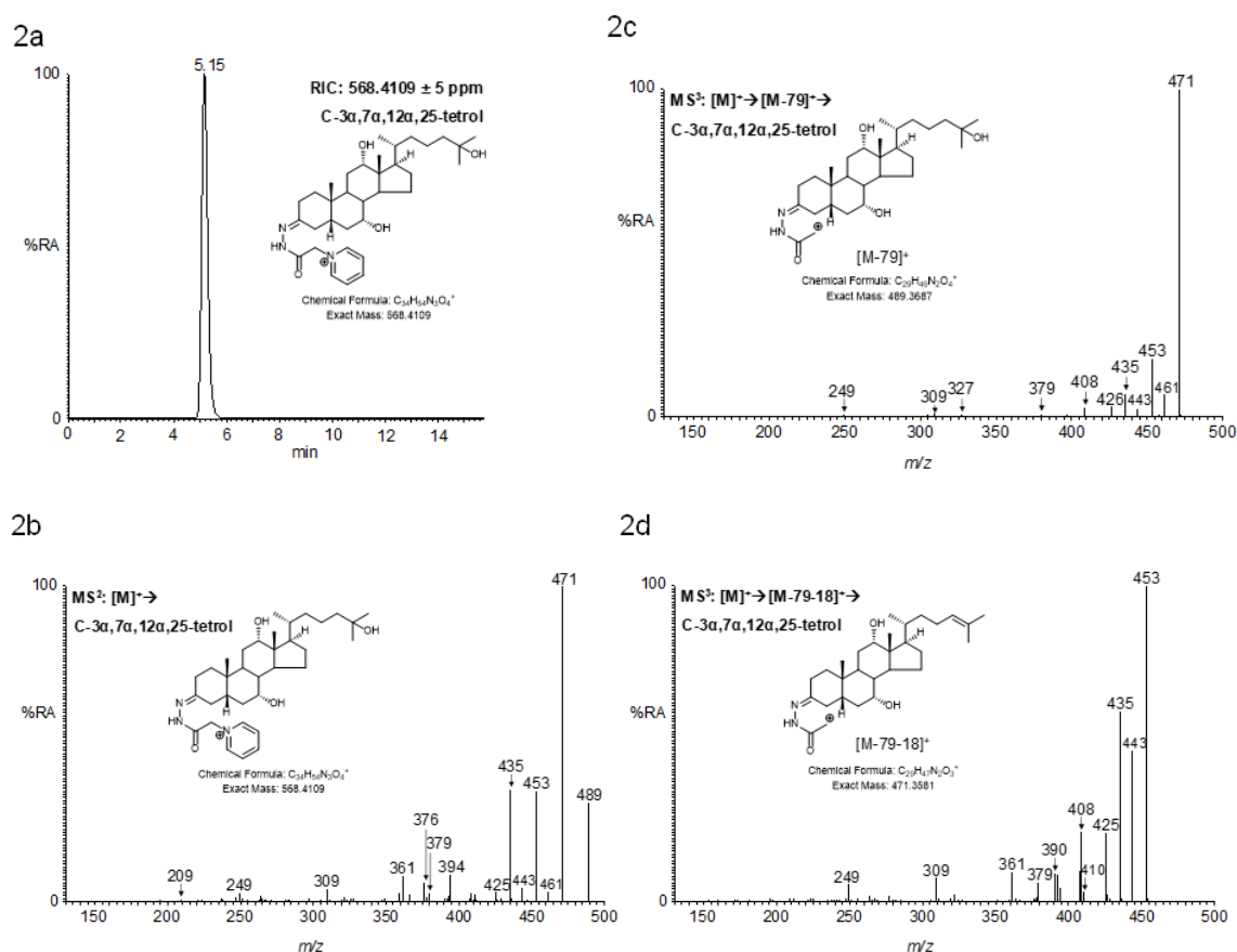
Figure 2. (a) RIC and (b) MS^2 ( [M]^+ \rightarrow ), (c) MS^3 ( [M]^+ \rightarrow [M-Py]^+ \rightarrow ), (d) ( [M]^+ \rightarrow [M-Py-18]^+ \rightarrow ) spectra of oxidized/GP-derivatized C-3 \alpha ,7 \alpha ,12 \alpha ,25-tetrol. For comparison, MS^2 ( [M]^+ \rightarrow ) spectra of C-3 \alpha ,7 \alpha ,12 \alpha -triol and C-3 \alpha ,7 \alpha ,12 \alpha ,26-tetrol and the MS^3 ( [M]^+ \rightarrow [M-Py-18]^+ \rightarrow ) spectrum of C-3 \alpha ,7 \alpha ,12 \alpha ,26-tetrol are shown in Supplemental Figures S1a, S1b, and S1c respectively. Mass spectra recorded at the peak of the RIC for these and other sterols analyzed are shown in Supplemental Figure S2. Data was generated on the Orbitrap-Elite mass spectrometer as in Figure 1. See Table 1 to correlate m/z with fragment ion composition.
