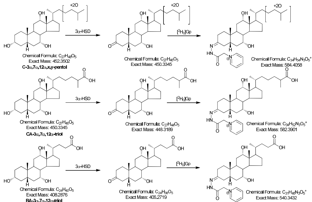
Scheme 2. Structures of bile alcohols and acids, and their products of 3 \alpha -HSD oxidation and GP-derivatization.
