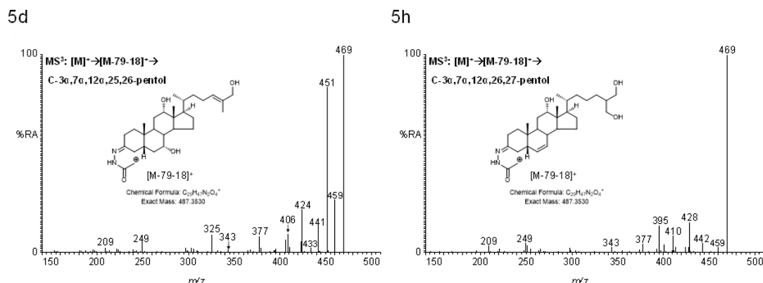
Figure 5. LC-(MS)MS n analysis of oxidized/GP-derivatized C-3 \alpha ,7 \alpha ,12 \alpha ,25,26-pentol and C-3 \alpha ,7 \alpha ,12 \alpha ,26,27-pentol: (a) RIC, (b) MS 2 ([M] + →), (c) MS 3 ([M] + →[M-Py] + →), and (d) ([M] + →[M-Py-18] + →) from the analysis of C-3 \alpha ,7 \alpha ,12 \alpha ,25,26-pentol. (e) RIC, (f) MS 2 ([M] + →), (g) MS 3 ([M] + →[M-Py] + →), and (h) ([M] + →[M-Py-18] + →) from the analysis of C-3 \alpha ,7 \alpha ,12 \alpha ,26,27-pentol. Data was generated on the Orbitrap-Elite mass spectrometer as in Figure 1. Fragment ions are described in Table 1 and postulated structures are shown in Supplemental Schemes S5 and S6.
