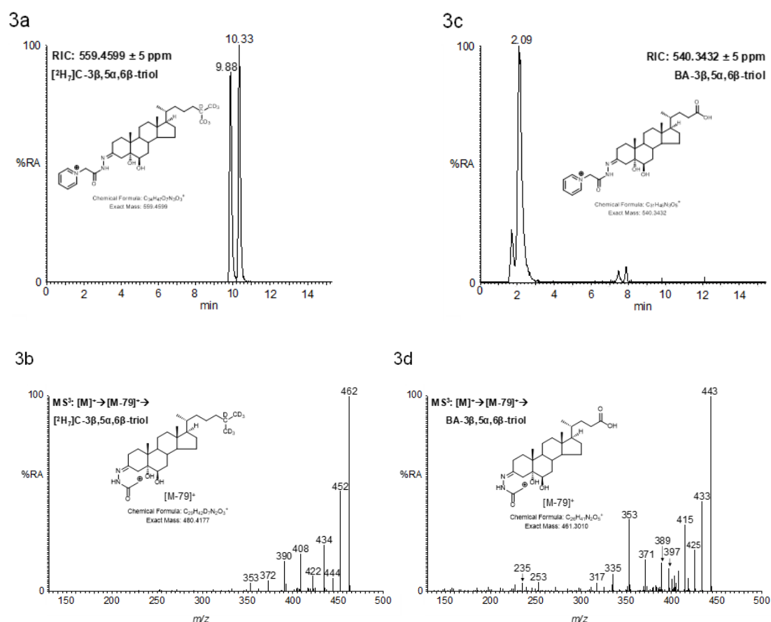
Figure 3. RICs and MS 3 ( [M]^+ \rightarrow [M-\text{Py}]^+ \rightarrow ) spectra of cholesterol oxidase-oxidized/GP-derivatized 3β,5α,6β-triols: (a,b) [25,26,26,26,27,27,27\text{-}^2\text{H}_7]\text{cholestane-}3\beta,5\alpha,6\beta\text{-triol} ( [^2\text{H}_7]\text{C-}3\beta,5\alpha,6\beta\text{-triol} ); (c,d) 3β,5α,6β-trihydroxycholanoic acid (BA-3β,5α,6β-triol). See reference [8] for a description of fragmentation pathways. GP-derivatized sterols can give syn and anti conformers resulting in twin chromatographic peaks which may or may not be resolved. Data was generated on the Orbitrap-Elite mass spectrometer as in Figure 1.
