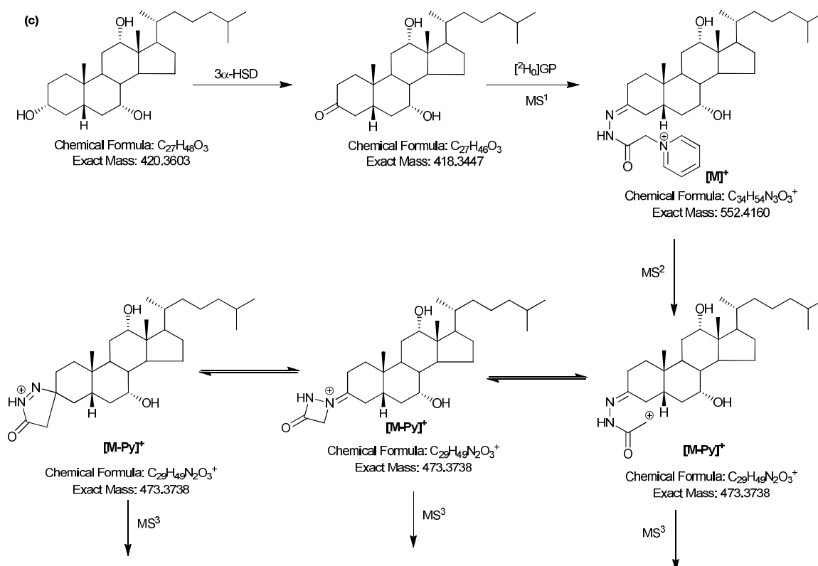
Scheme 1. Enzyme-assisted derivatization for sterol analysis (EASDA): (a) EADSA of the 3 \beta -hydroxy-5-ene function using cholesterol oxidase and [^2H_5] Girard P reagent ( [^2H_5]GP ); (b) derivatization of the 3-oxo-4-ene function with [^2H_0]GP ; (c) EADSA of the 3 \alpha -hydroxy-5 \beta -hydrogen function with 3 \alpha -hydroxysteroid dehydrogenase (3 \alpha -HSD) and [^2H_0]GP . Derivatives with the [^2H_5]GP and [^2H_0]GP reagents can be combined and analyzed in a single LC-MS run. Other isotope-coded GP reagents have been synthesized to allow triplex analysis if required [45].
