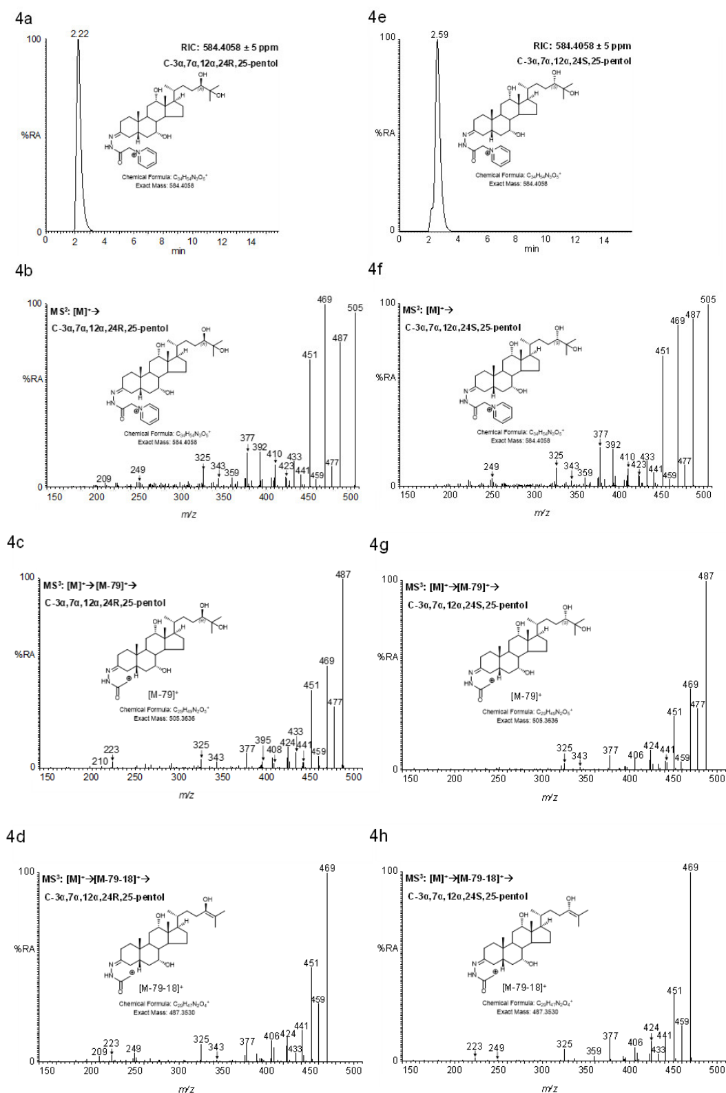
Figure 4. LC-(MS)MS n analysis of oxidized/GP-derivatized C-3α,7α,12α,24R,25-pentol and C-3α,7α,12α,24S,25-pentol: (a) RIC, (b) MS 2 ([M] + →), (c) MS 3 ([M] + →[M-Py] + →), and (d) ([M] + →[M-Py-18] + →) from the analysis of C-3α,7α,12α,24R,25-pentol. (e) RIC, (f) MS 2 ([M] + →), (g) MS 3 ([M] + →[M-Py] + →), and (h) ([M] + →[M-Py-18] + →) from the analysis of C-3α,7α,12α,24S,25-pentol. Data was generated on the Orbitrap-Elite mass spectrometer as in Figure 1. Fragment ions are described in Table 1 and postulated structures are shown in Scheme 4.
