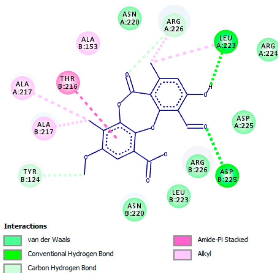
Figure 4. Molecular interaction of psoromic acid (PA) with the active site of HSV-2 protease. Amino acid residues involved in HSV-2 protease stabilization along with the hydrogen bonding and other essential interactions for enzyme inactivation are illustrated. Significant functional groups of PA that account for the inhibitory action against HSV-2 protease are presented.
