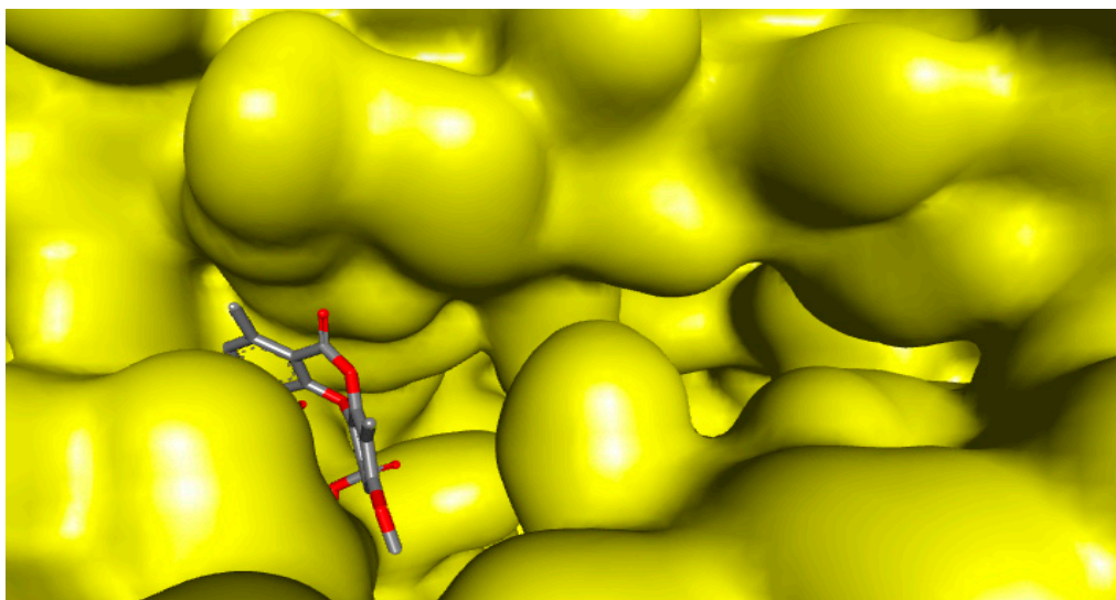
Figure 3. Molecular surface depiction of HSV-2 protease. As shown, psoromic acid binds remarkably to the active site of the enzyme.
