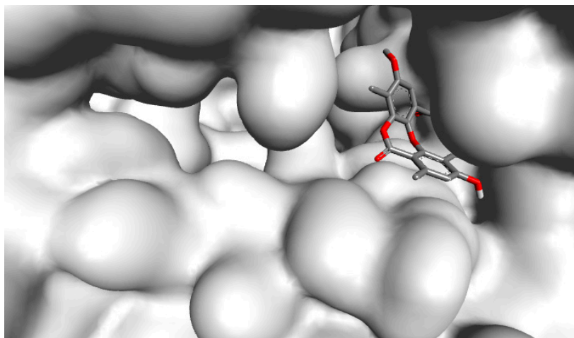
Figure 1. Molecular surface illustration of HSV-1 DNA polymerase, where psoromic acid efficiently binds to the active site of the enzyme.
