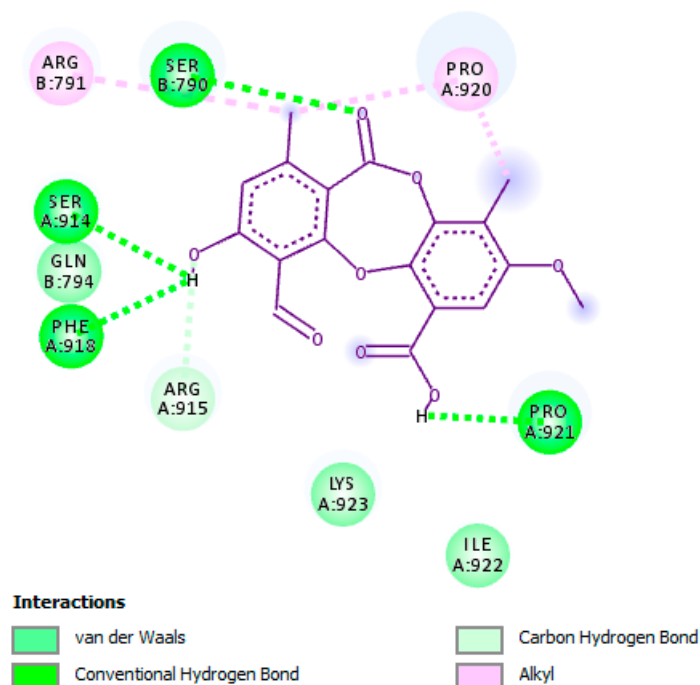
Figure 2. Molecular interaction of psoromic acid (PA) with the active site of HSV-1 DNA polymerase. Amino acid residues involved in HSV-1 DNA polymerase stabilization along with the hydrogen bonding and other essential interactions for enzyme inactivation are presented. The key functional groups of PA that are responsible for anti-HSV-1 DNA polymerase activity are depicted.
