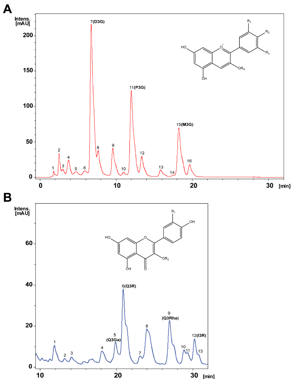
Figure 1. Representative chromatographic analysis of Calafate berry extracts. (A) Prototype anthocyanins chromatogram of the hydroalcoholic extract based on 520 nm absorbance. Sixteen major peaks were observed; mass spectra analysis of the peaks revealed the list of putative compounds shown in Table 1. Inset shows the basic anthocyanin structure; position 3 conjugations are referred to as R_4 substituents. (B) Representative chromatogram of hydroalcoholic extract flavonols identified by absorbance at 360 nm; the 13 major peaks identified and analyzed by mass spectrum are listed in Table 1. The basic flavonols structure and its glycosylated substituents in R_2 refer to the various sugar conjugates present in the extract.
