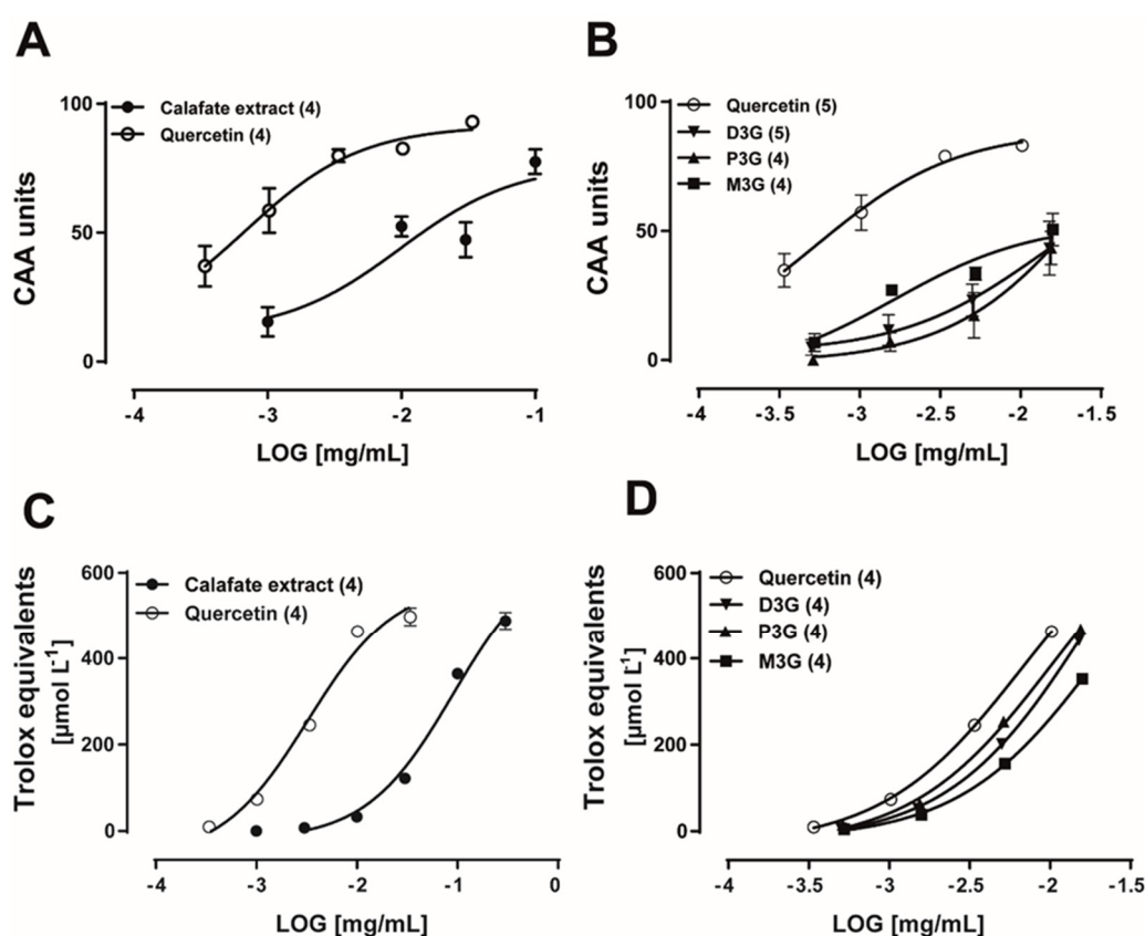
Figure 3. Comparison of the antioxidant activity of the extract and major extract anthocyanins by two methods: the cellular antioxidant activity (CAA) versus the DPPH assay. (A) Calafate extract and quercetin control antioxidant concentration–response curves. (B) Antioxidant effect of the three major Calafate anthocyanins in the CAA assay measured in endothelial cells examined in the same concentration range that caused vasodilatation. Calafate extract antioxidant activity measured by the DPPH assay and its comparison with quercetin (C) or the three major extract anthocyanins (D). Symbols represent the mean values, bars the SEM. While the CAA activity is expressed in relative units, the DPPH assay is expressed in Trolox equivalents.
