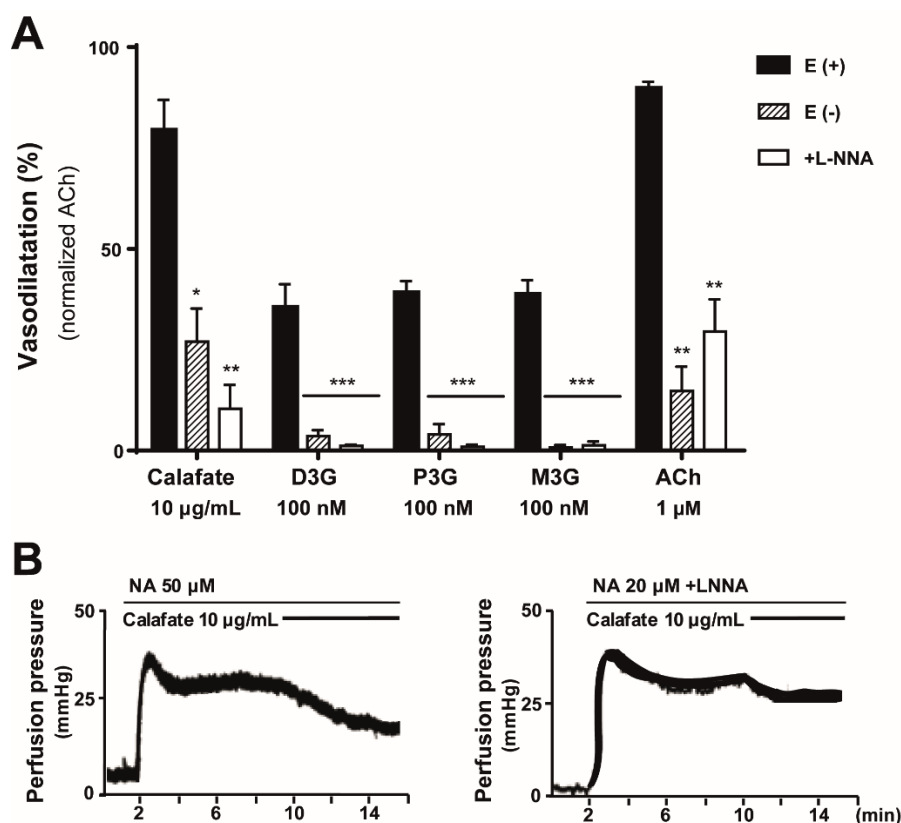
Figure 4. Endothelium-dependent mechanism of the Calafate extract and anthocyanin vasodilation; endothelial nitric oxide synthase enzyme (eNOS) participation. (A) The vasodilatation elicited by 10\mu\text{g/mL} extract ( n = 10 ) or 100\text{ nM} of delphinidin-3-glucoside (D3G, n = 6 ), petunidin-3-glucoside (P3G, n = 6 ), malvidin-3-glucoside (M3G, n = 4 ), or acetylcholine (ACh, n = 19 ) perfused in intact mesenteries or by the same mesentery devoid of endothelium (-). In parallel, separate protocols evaluated the role of eNOS activity after enzyme blockade following tissue perfusion with 150\mu\text{M} L-NNA. Vasorelaxations were normalized by the 1\mu\text{M} ACh-induced vasodilation. Columns denote the mean values, bars the SEM. *, p < 0.05 , **, p < 0.01 , ***, p < 0.001 (B) Representative tracings of the vasodilatation elicited by 10\mu\text{g/mL} Calafate extract before (control) and following eNOS inhibition with L-NNA. Note that after L-NNA treatment, the concentration of NA was reduced to 20\mu\text{M} , because of tissue sensitization.
