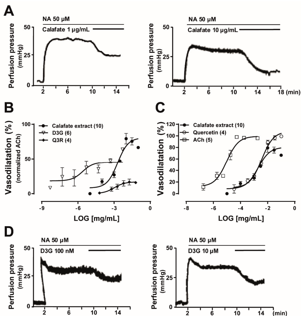
Figure 2. Concentration-dependent vasodilatation induced by Calafate berry extracts and the mimetic action of delphinidin-3-glucoside, quercetin, quercetin-3-rutinoside or acetylcholine in the rat arterial mesenteric bed. (A) Representative tracings of the hydroalcoholic extract-induced vasodilatation elicited by perfusion with 1 or 10 µg/mL; the extract was dissolved in distilled water and diluted in perfusion buffer. (B) The normalized 1 µM ACh concentration-dependent vasodilatation curves of the hydroalcoholic extract (solid circles) were compared to the main anthocyanin (delphinidin-3-glucoside, D3G open triangle) or flavonol (quercetin-3-rutinoside, Q3R solid diamond). (C) Comparison of the vasodilatation elicited by the Calafate extract, quercetin (open circles) or acetylcholine (ACh, open square). Symbols represent the mean values; bars the SEM. The number in parenthesis of panels B and C represents protocol replicates. (D) Representative tracings of the vasodilator response induced by 100 nM and 10 µM delphinidin-3-glucoside (D3G). All the experiments were made in intact mesenteric beds (with endothelium).
