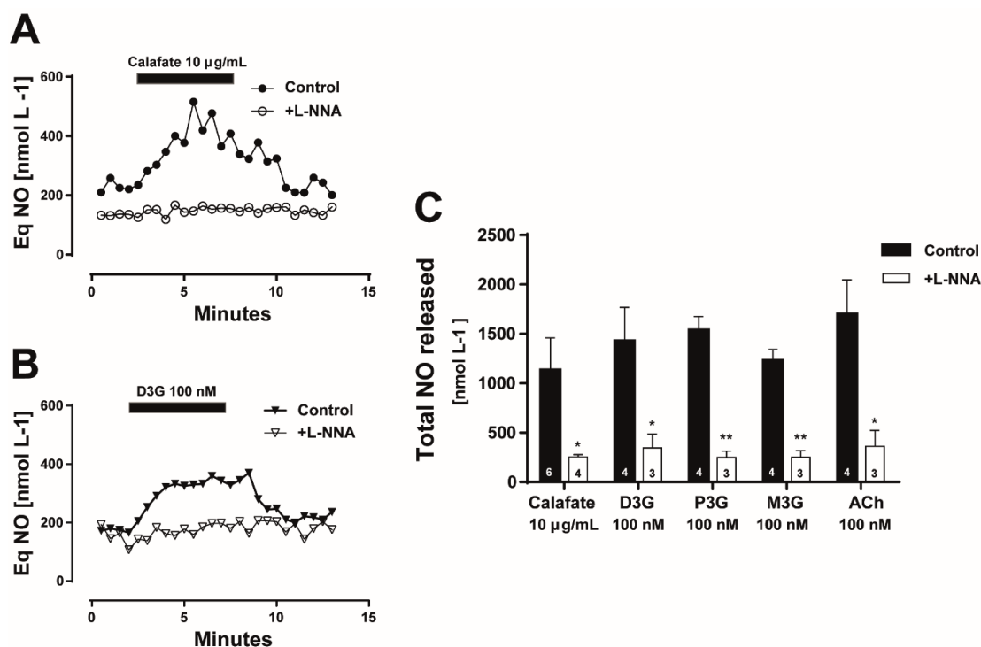
Figure 5. Luminally accessible NO determinations elicited by Calafate extract perfusion or the main anthocyanins. (A) Representative time course of NO released to the perfusate following 10 \mu g/mL Calafate extract application (closed symbols) and following eNOS blockade with 150 \mu M L-NNA (open symbols) in the same preparation. (B) Representative time course of luminally accessible NO elicited by perfusion with 100 nM of delphinidin-3-glucoside (D3G) in a control preparation (closed symbols) and following L-NNA (open symbols). (C) Statistical analysis of NO production elicited by perfusion with 10 \mu g/mL Calafate extract, 100 nM delphinidin-3-glucoside (D3G), petunidin-3-glucoside (P3G), malvidin-3-glucoside (M3G) and acetylcholine (ACh) before and after treatment with the enzyme inhibitor. Columns represent the mean values; bars the SEM. The number inside the columns represents protocol repetitions in separate mesenteries. *, p < 0.05 ; **, p < 0.01 .
