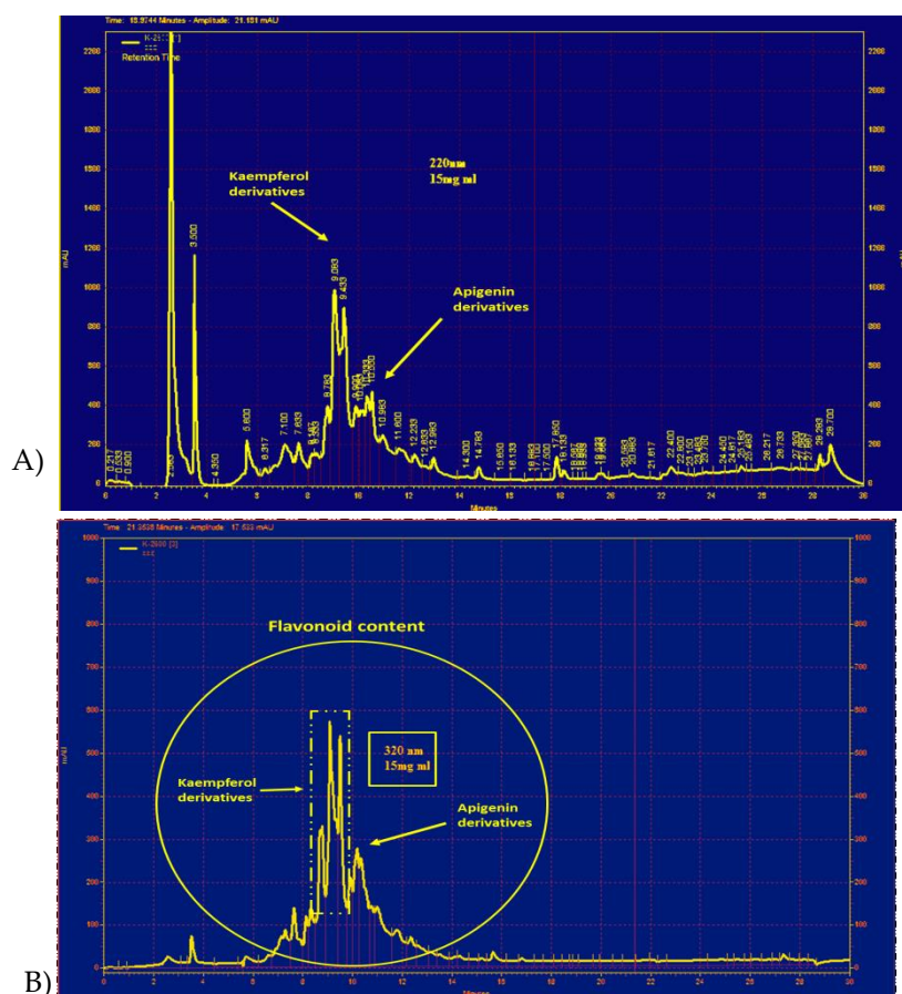
Figure 6. HPLC fingerprint of the hydro-ethanollic extract of P. oleracea at 220 nm (A) and 320 nm (B) (reprinted with permission from Ref. [20]).
