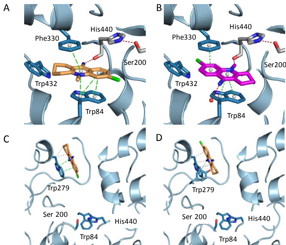
Figure 2. Binding mode of 5 within the TcAChE active site ( A,B ), and at the PAS ( C,D ). In the active site, the major pose is represented in ( A ), with the conjugated system of 5 \pi -stacked between Phe330 and Trp84. However, the Cl atom does not point towards Trp432, as usually observed for 6-chlorotacrine derivatives, and the nitrogen of the exocyclic amino group is H-bonded to the carbonyl group of catalytic His440. A minor pose has also been modeled, with the Cl atom towards the hydrophobic pocket. In this orientation, the methyl group makes close contact (2.7 Å) with catalytic His440, and potentially interacts via a weak H-bond [45]. At the peripheral site, two orientations are also observed, and were refined with identical occupancies (0.5). Hydrophobic interactions are represented as dashed gray lines, \pi -stacking interactions are in green, and hydrogen bonds are in red.
