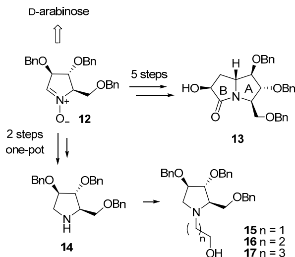
Scheme 1. Synthetic steps to access pyrrolizidine lactam 13 and hydroxypyrrolidines 15–17 (through the key intermediate 14 ) from nitron 12 .
