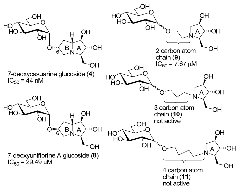
Figure 3. Compounds 4 , 8 , 9 , 10 , 11 and their IC_{50} values towards C. riparius trehalase.
