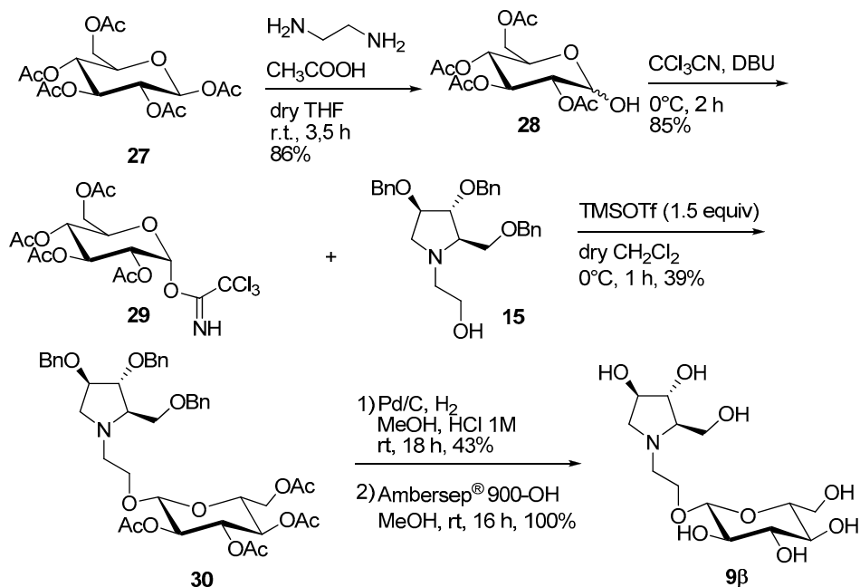
Scheme 4. Synthesis of the pseudodisaccharide 9 \beta .
