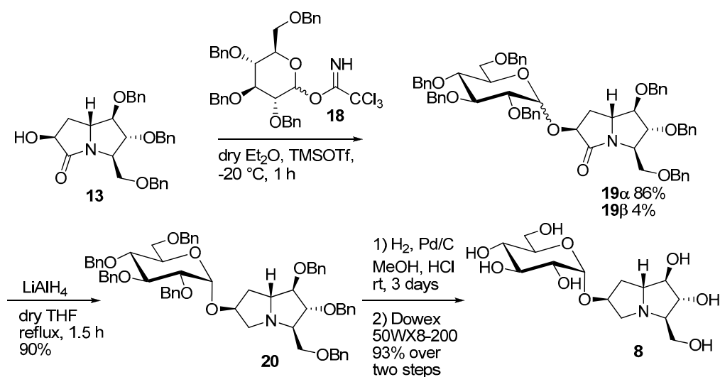
Scheme 2. Synthesis of the pseudodisaccharide 7-deoxyuniflorine A glucoside ( 8 ).
