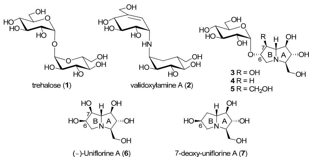
Figure 1. Trehalose (1), the natural substrate of the enzyme \alpha -trehalase (EC 3.2.1.28), and some natural and non-natural trehalase inhibitors reported to date.
