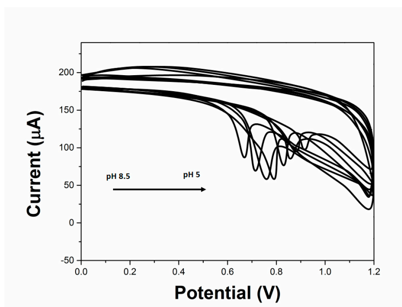
Figure S1. CVs of 0.1 mM MT obtained at GNs/HA/GCE at pH conditions from 5.0 to 8.5.
