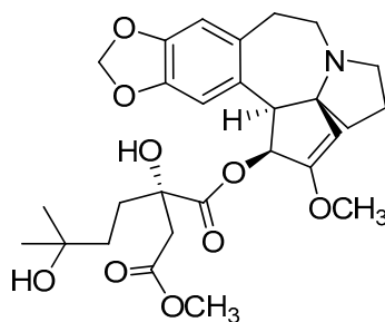
Harringtonine ( 68 )
