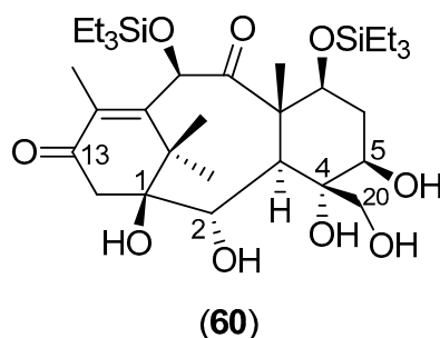
Figure 11. Structure of Compound 60.
