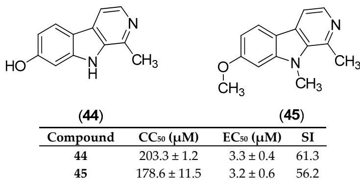
Figure 8. \beta -Carbolines harmol (Compound 44) and its synthetic derivative 9- N -methylharmine (Compound 45).
