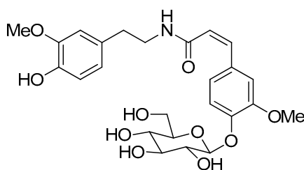
Drodrenin ( 71 )
