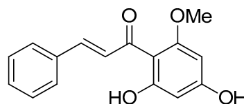
Cardamonin (4)
