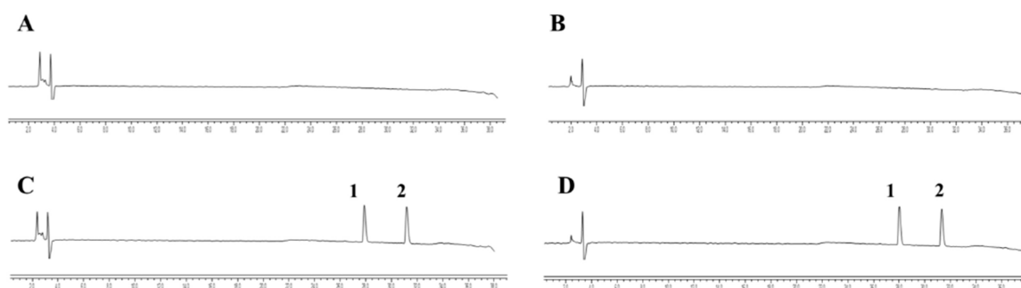
Figure S1. Representative HPLC chromatographic profiles: (A) blank-HLM reaction system. (B) blank-mixed rCYPs reaction system. (C) norCLZ and CLZ N -oxide-HLM reaction system. (D) norCLZ and CLZ N -oxide - mixed rCYPs reaction system. 1, norCLZ; 2, CLZ N -oxide.
