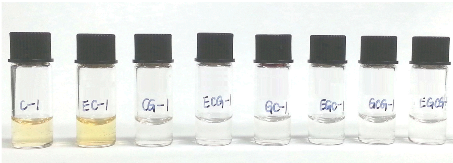
Figure S1. The picture of aqueous solutions of 8 catechins (575 \mu\text{M} ) after 15-day-storage under laboratory illumination at 25 °C.
