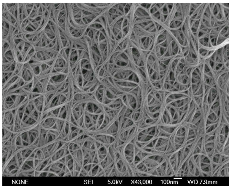
Figure S2. SEM characterization of purified CNT film.
