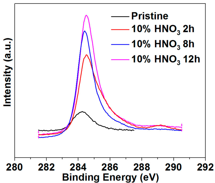
Figure S3. C (1s) XPS scan results of different HNO 3 etching duration samples.
