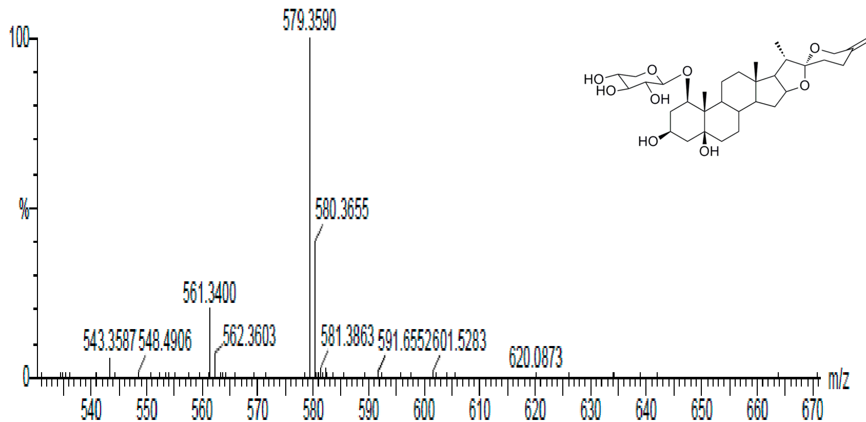
Figure S17. The HR-ESI-MS spectrum of 3 (in MeOH).
