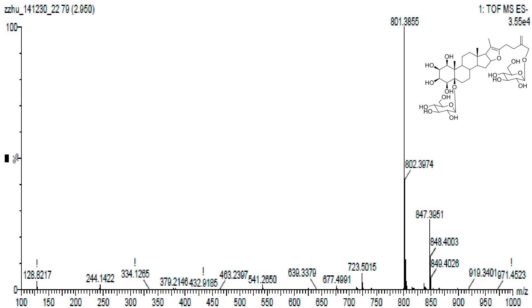
Figure S2. The HR-ESI-MS spectrum of 1 (in MeOH).
