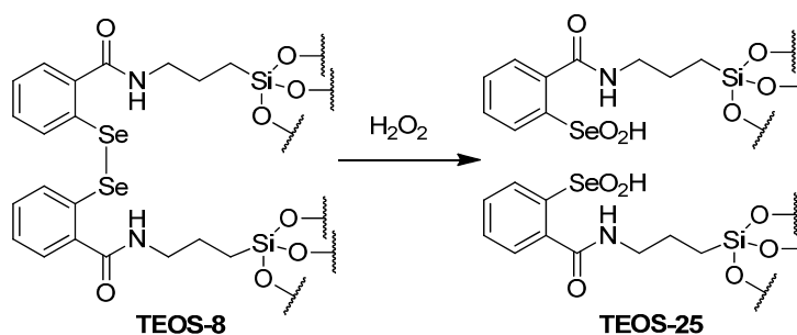
Scheme 6. Oxidation of TEOS-8 with \text{H}_2\text{O}_2 to seleninic-acid containing TEOS-25 .
