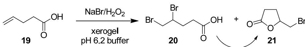
Scheme 3. Bromination of 4-pentenoic acid ( 19 ) as an indirect measure of bromine/hypobromous acid production from the oxidation of bromide with hydrogen peroxide.
