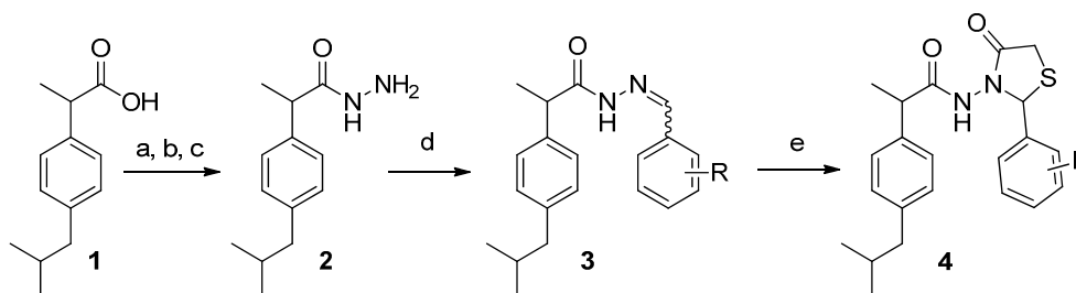
Scheme 1. Synthetic procedure of compounds 4a–n .
