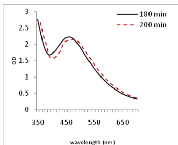
Figure 1. UV-visible absorption spectra of Ab.Ag-NPs in different times.
