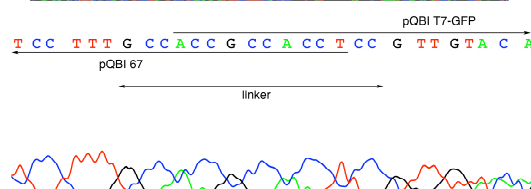
Supporting Figure 1. Sequencing of the recombinant plasmids. (a) A GFP-recombinant. (b) A BFP-recombinant. (c) One of the fusion recombinant.
